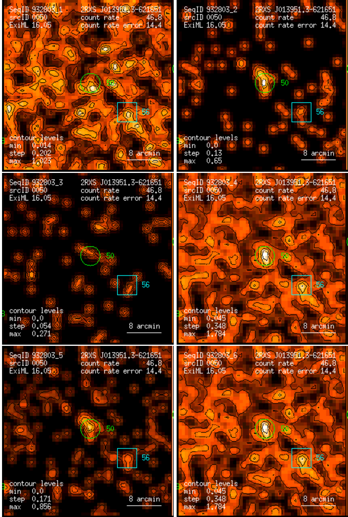
Figure 50: RASS 932803: detection 0050: band rate images, Gaussian filter: (1) PSPC channels 11 – 41, (2) 52 – 90, (3) 91 – 201, (4) 11 – 235, (5) 52 – 201, (6) 11 – 201. Broad band rates in counts/ks. Band rate contour levels in counts/ks/arcmin 2 .
