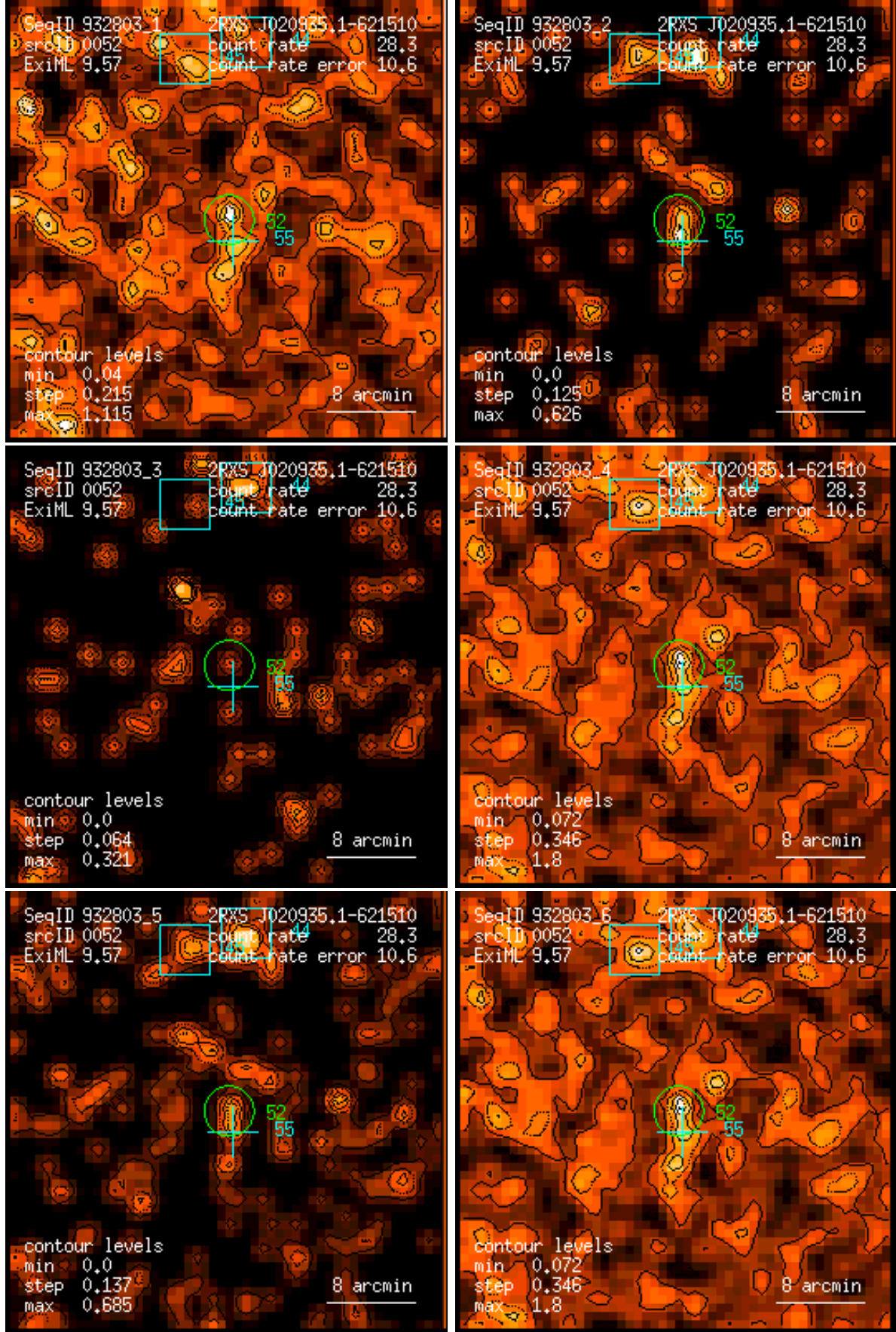
Figure 52: RASS 932803: detection 0052: band rate images, Gaussian filter: (1) PSPC channels 11 – 41, (2) 52 – 90, (3) 91 – 201, (4) 11 – 235, (5) 52 – 201, (6) 11 – 201. Broad band rates in counts/ks. Band rate contour levels in counts/ks/arcmin 2 .
