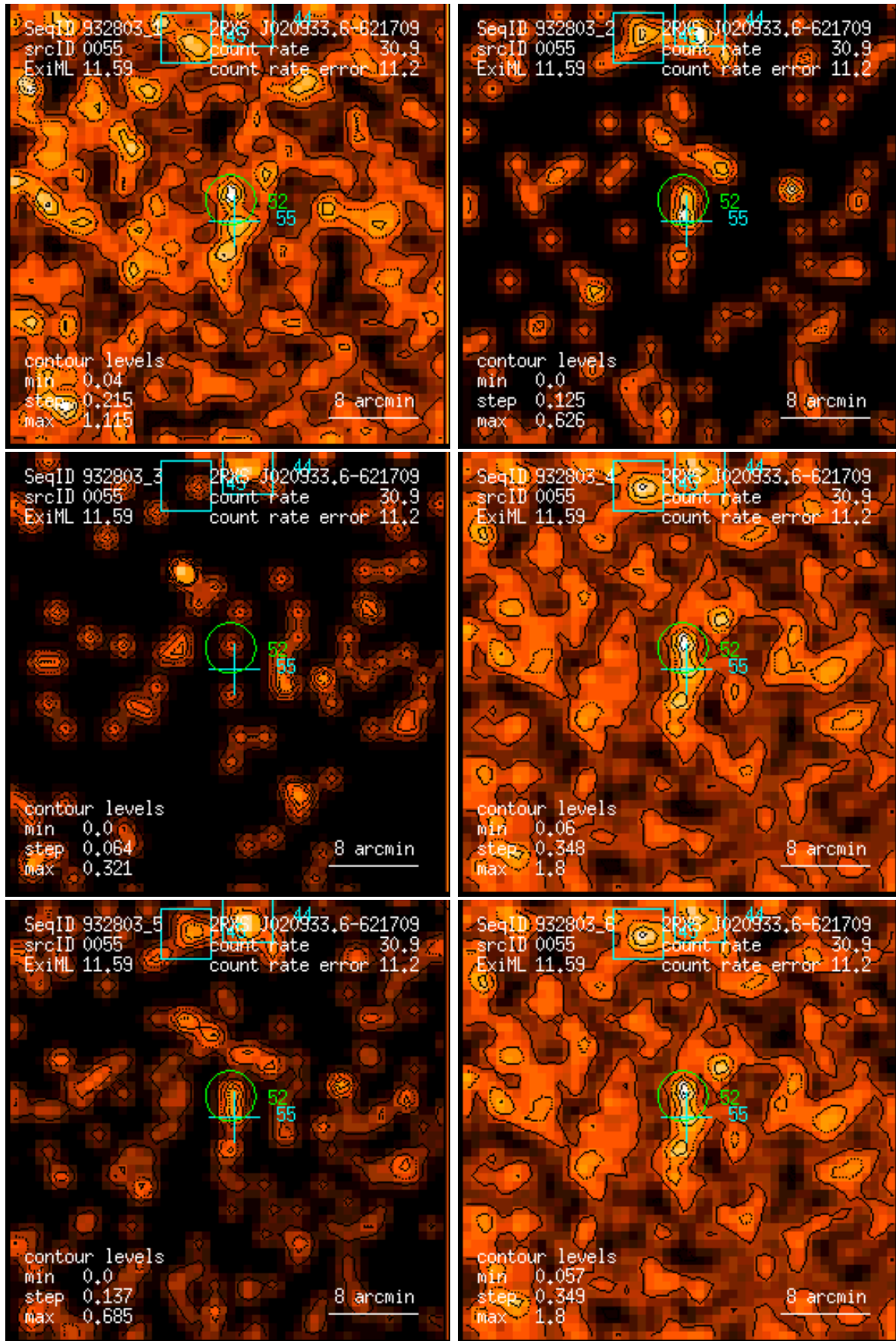
Figure 55: RASS 932803: detection 0055: band rate images, Gaussian filter: (1) PSPC channels 11 – 41, (2) 52 – 90, (3) 91 – 201, (4) 11 – 235, (5) 52 – 201, (6) 11 – 201. Broad band rates in counts/ks. Band rate contour levels in counts/ks/arcmin 2 .
