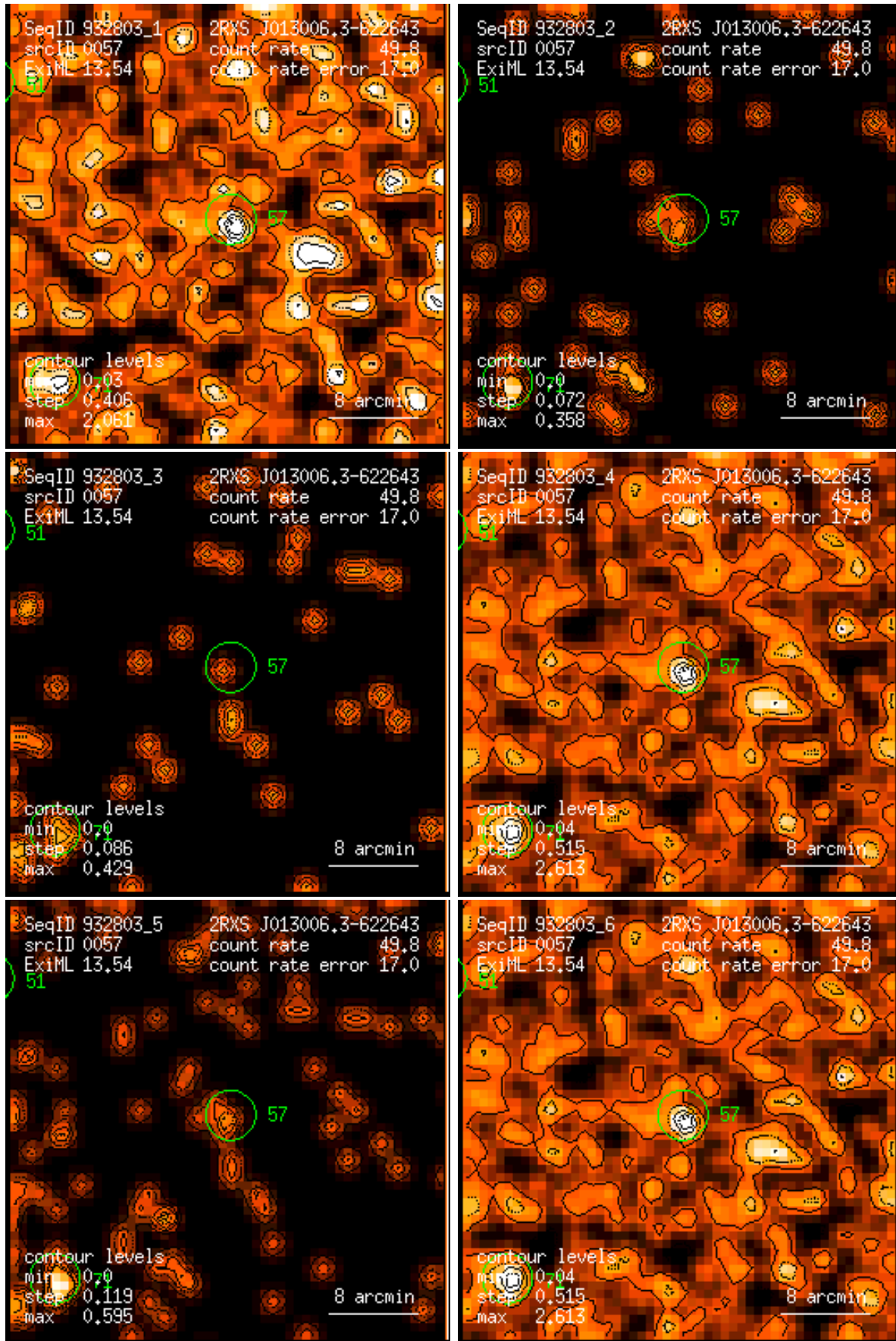
Figure 57: RASS 932803: detection 0057: band rate images, Gaussian filter: (1) PSPC channels 11 – 41, (2) 52 – 90, (3) 91 – 201, (4) 11 – 235, (5) 52 – 201, (6) 11 – 201. Broad band rates in counts/ks. Band rate contour levels in counts/ks/arcmin 2 .
