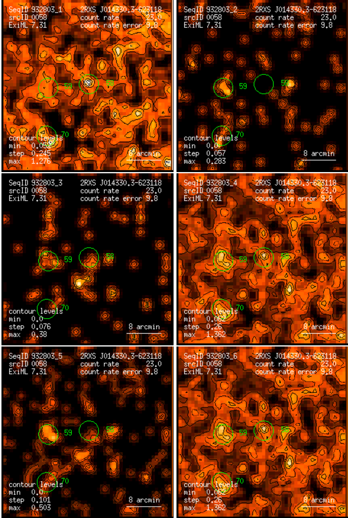
Figure 58: RASS 932803: detection 0058: band rate images, Gaussian filter: (1) PSPC channels 11 – 41, (2) 52 – 90, (3) 91 – 201, (4) 11 – 235, (5) 52 – 201, (6) 11 – 201. Broad band rates in counts/ks. Band rate contour levels in counts/ks/arcmin 2 .
