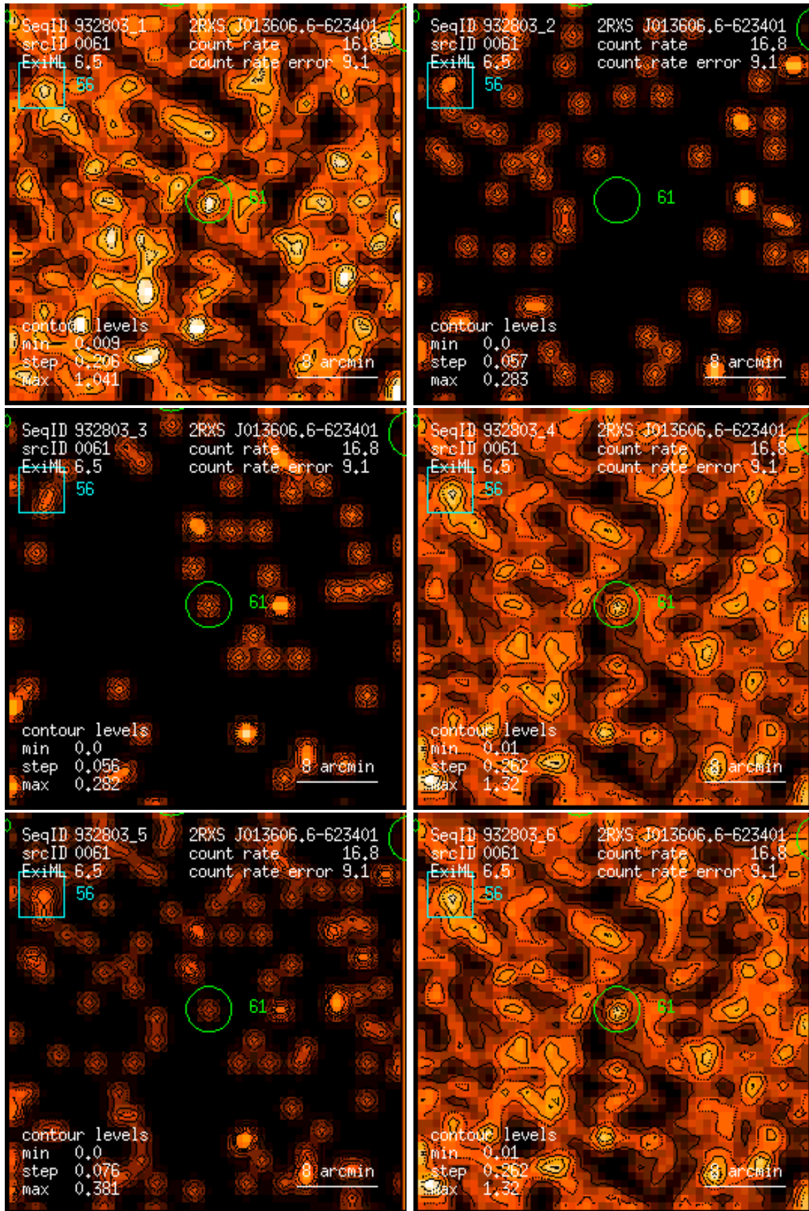
Figure 61: RASS 932803: detection 0061: band rate images, Gaussian filter: (1) PSPC channels 11 – 41, (2) 52 – 90, (3) 91 – 201, (4) 11 – 235, (5) 52 – 201, (6) 11 – 201. Broad band rates in counts/ks. Band rate contour levels in counts/ks/arcmin 2 .
