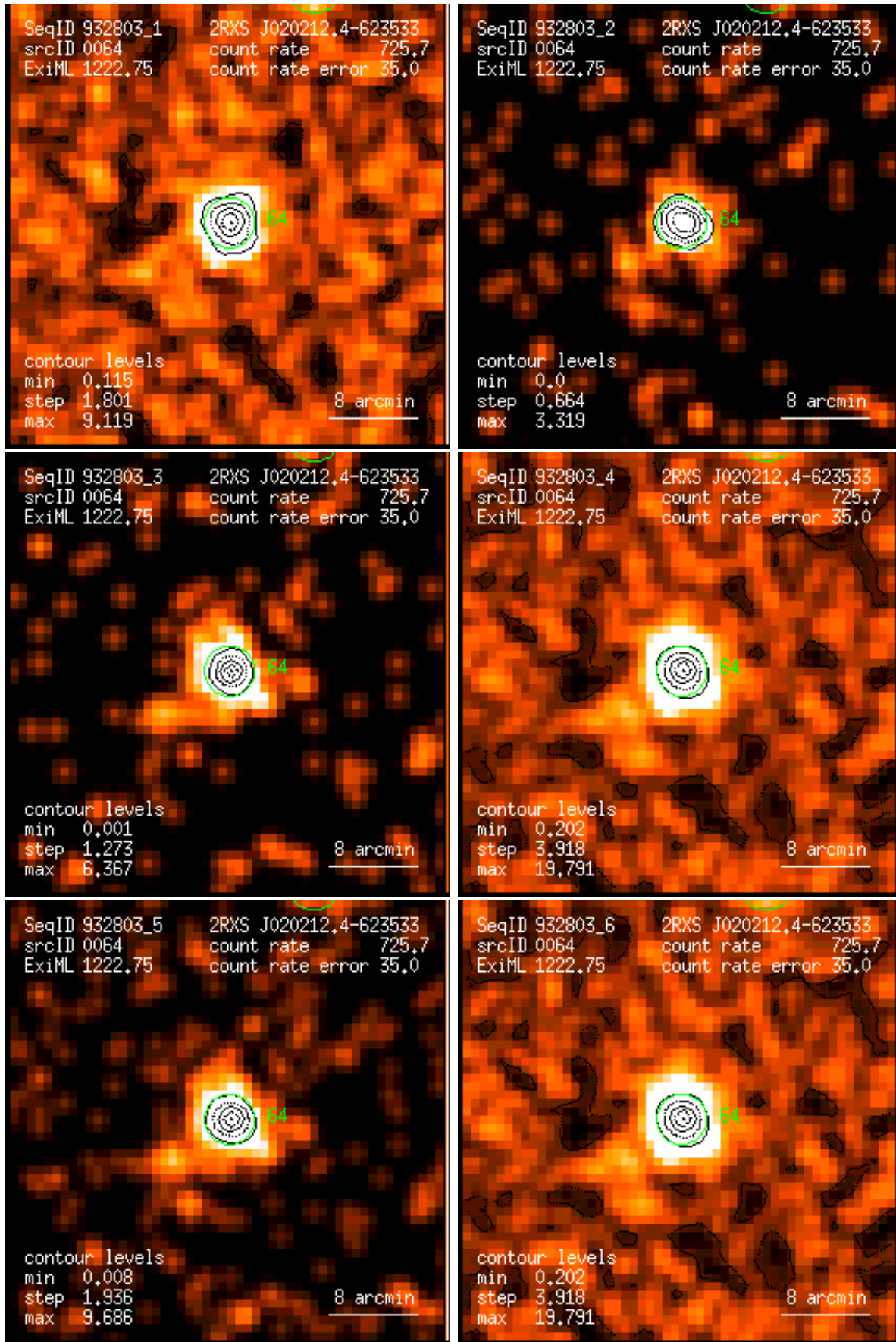
Figure 64: RASS 932803: detection 0064: band rate images, Gaussian filter: (1) PSPC channels 11 – 41, (2) 52 – 90, (3) 91 – 201, (4) 11 – 235, (5) 52 – 201, (6) 11 – 201. Broad band rates in counts/ks. Band rate contour levels in counts/ks/arcmin 2 .
