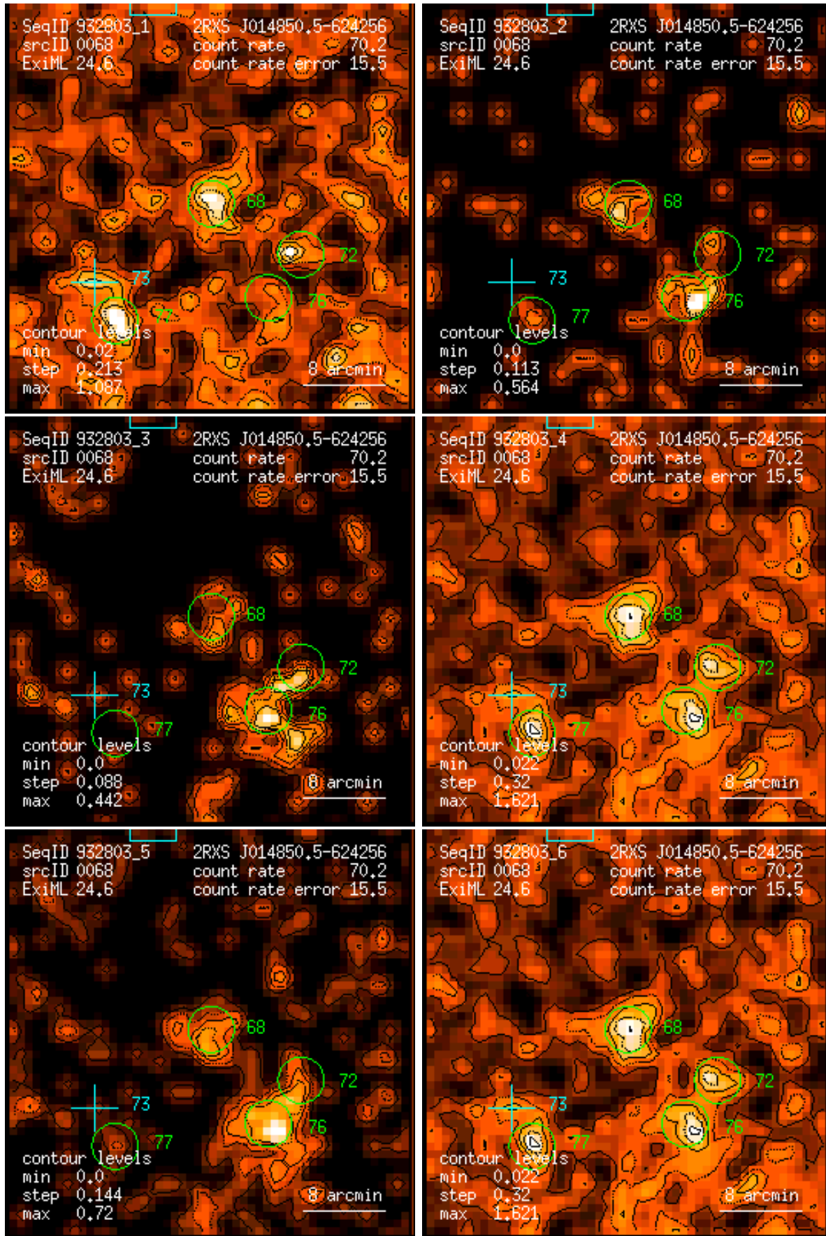
Figure 68: RASS 932803: detection 0068: band rate images, Gaussian filter: (1) PSPC channels 11 – 41, (2) 52 – 90, (3) 91 – 201, (4) 11 – 235, (5) 52 – 201, (6) 11 – 201. Broad band rates in counts/ks. Band rate contour levels in counts/ks/arcmin 2 .
