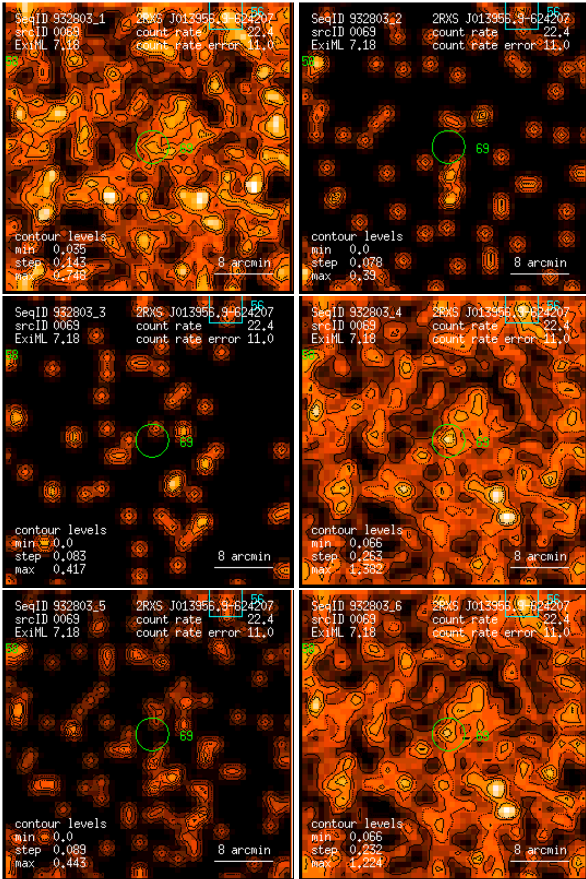
Figure 69: RASS 932803: detection 0069: band rate images, Gaussian filter: (1) PSPC channels 11 – 41, (2) 52 – 90, (3) 91 – 201, (4) 11 – 235, (5) 52 – 201, (6) 11 – 201. Broad band rates in counts/ks. Band rate contour levels in counts/ks/arcmin 2 .
