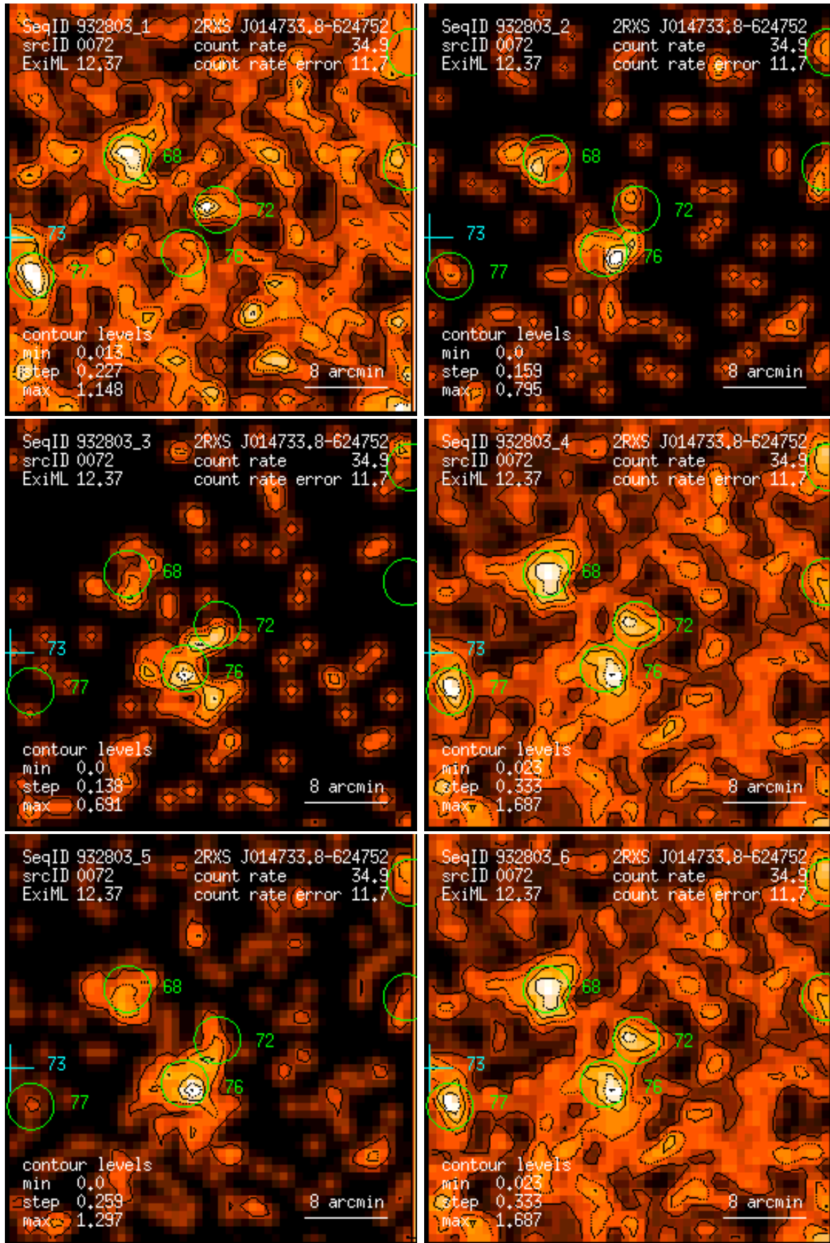
Figure 72: RASS 932803: detection 0072: band rate images, Gaussian filter: (1) PSPC channels 11 – 41, (2) 52 – 90, (3) 91 – 201, (4) 11 – 235, (5) 52 – 201, (6) 11 – 201. Broad band rates in counts/ks. Band rate contour levels in counts/ks/arcmin 2 .
