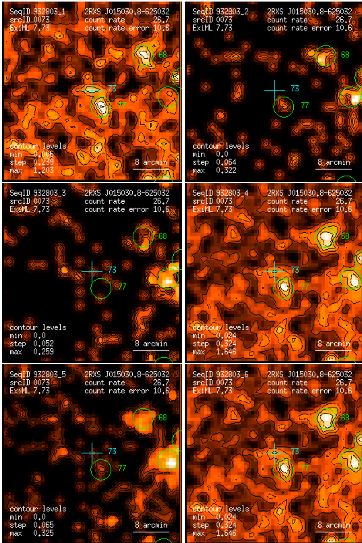
Figure 73: RASS 932803: detection 0073: band rate images, Gaussian filter: (1) PSPC channels 11 – 41, (2) 52 – 90, (3) 91 – 201, (4) 11 – 235, (5) 52 – 201, (6) 11 – 201. Broad band rates in counts/ks. Band rate contour levels in counts/ks/arcmin 2 .
