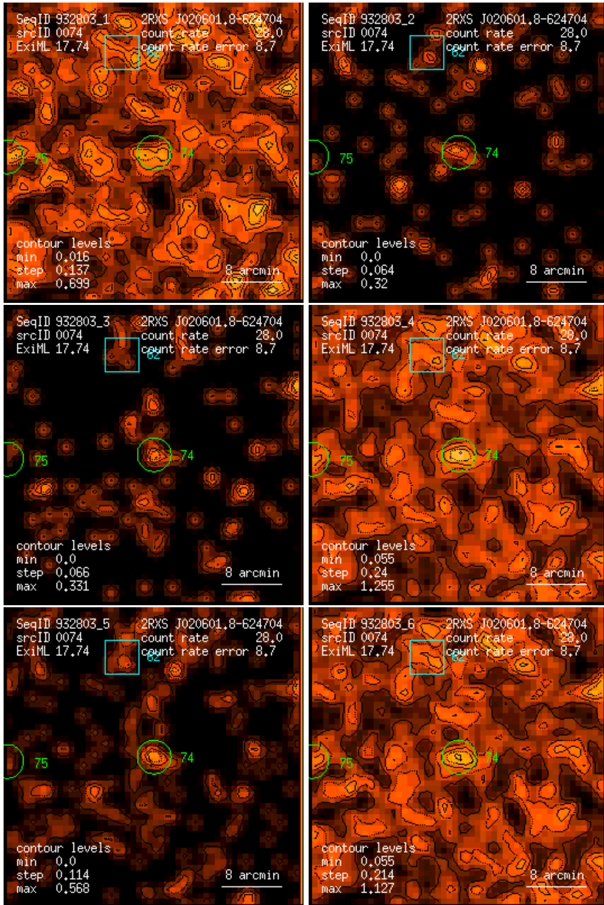
Figure 74: RASS 932803: detection 0074: band rate images, Gaussian filter: (1) PSPC channels 11 – 41, (2) 52 – 90, (3) 91 – 201, (4) 11 – 235, (5) 52 – 201, (6) 11 – 201. Broad band rates in counts/ks. Band rate contour levels in counts/ks/arcmin 2 .
