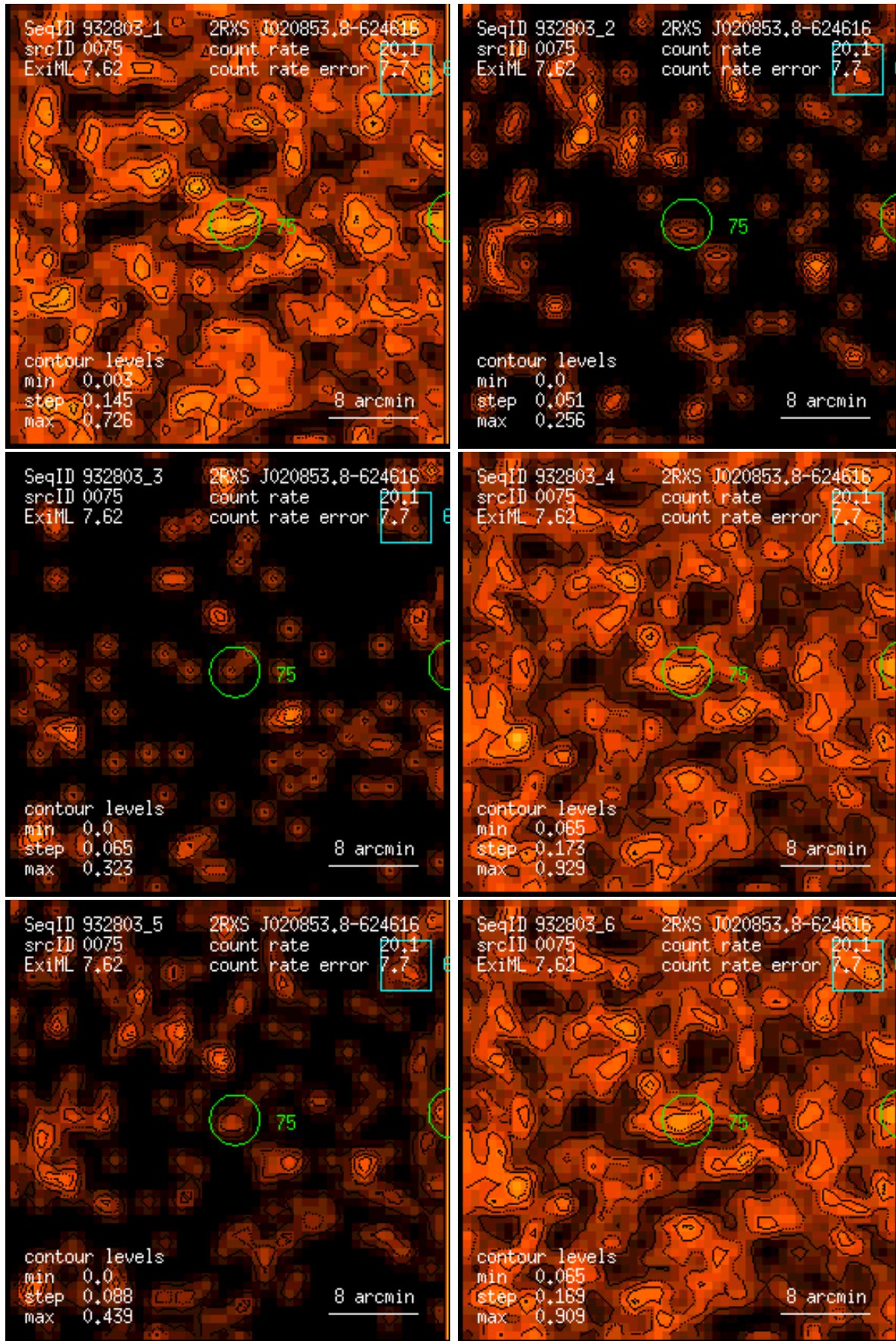
Figure 75: RASS 932803: detection 0075: band rate images, Gaussian filter: (1) PSPC channels 11 – 41, (2) 52 – 90, (3) 91 – 201, (4) 11 – 235, (5) 52 – 201, (6) 11 – 201. Broad band rates in counts/ks. Band rate contour levels in counts/ks/arcmin 2 .
