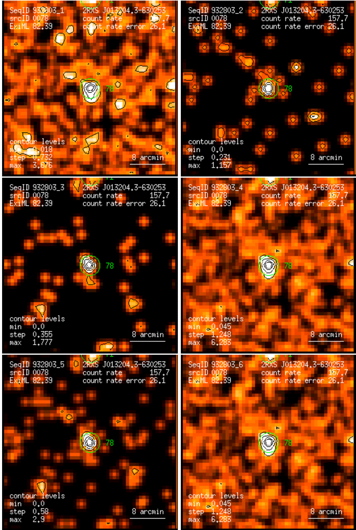
Figure 78: RASS 932803: detection 0078: band rate images, Gaussian filter: (1) PSPC channels 11 – 41, (2) 52 – 90, (3) 91 – 201, (4) 11 – 235, (5) 52 – 201, (6) 11 – 201. Broad band rates in counts/ks. Band rate contour levels in counts/ks/arcmin 2 .
