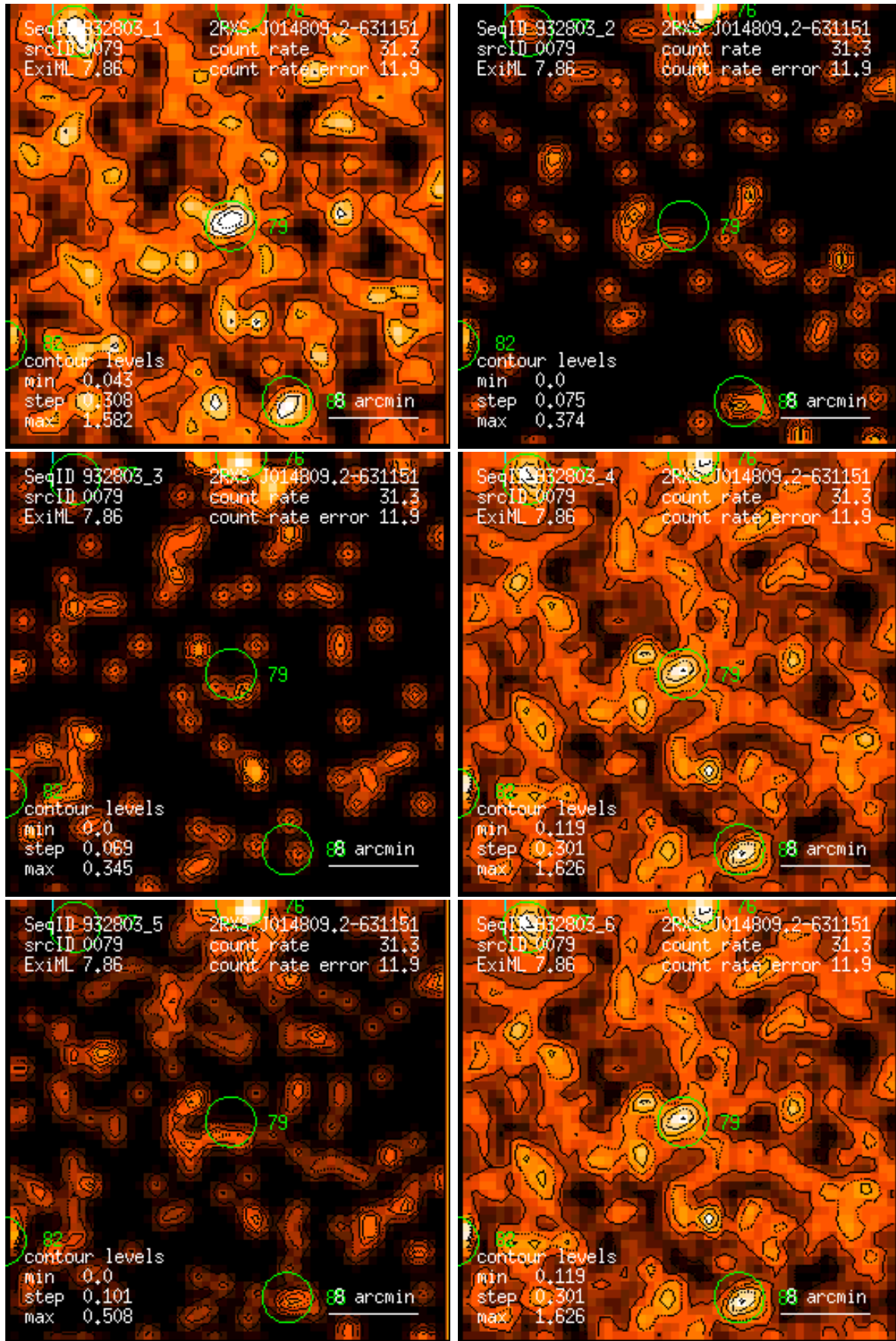
Figure 79: RASS 932803: detection 0079: band rate images, Gaussian filter: (1) PSPC channels 11 – 41, (2) 52 – 90, (3) 91 – 201, (4) 11 – 235, (5) 52 – 201, (6) 11 – 201. Broad band rates in counts/ks. Band rate contour levels in counts/ks/arcmin 2 .
