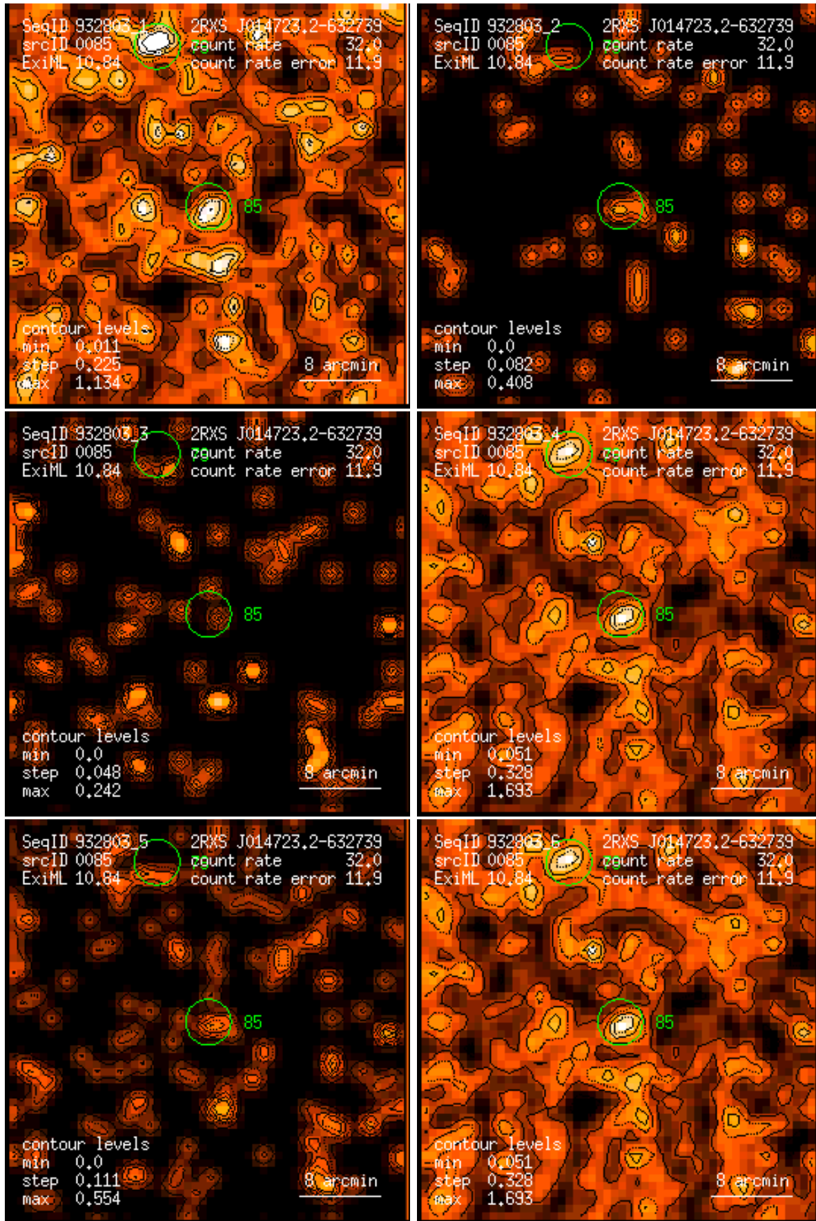
Figure 85: RASS 932803: detection 0085: band rate images, Gaussian filter: (1) PSPC channels 11 – 41, (2) 52 – 90, (3) 91 – 201, (4) 11 – 235, (5) 52 – 201, (6) 11 – 201. Broad band rates in counts/ks. Band rate contour levels in counts/ks/arcmin 2 .
