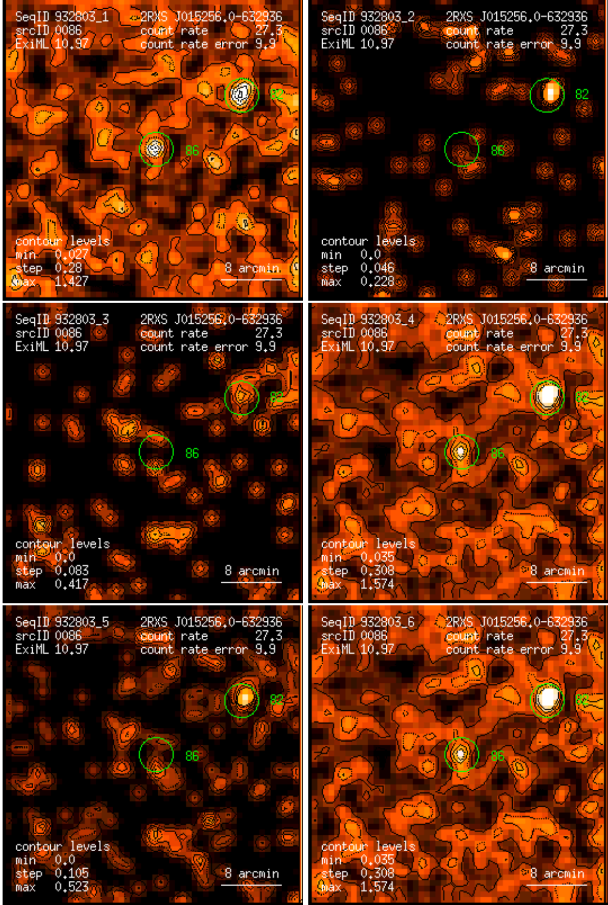
Figure 86: RASS 932803: detection 0086: band rate images, Gaussian filter: (1) PSPC channels 11 – 41, (2) 52 – 90, (3) 91 – 201, (4) 11 – 235, (5) 52 – 201, (6) 11 – 201. Broad band rates in counts/ks. Band rate contour levels in counts/ks/arcmin 2 .
