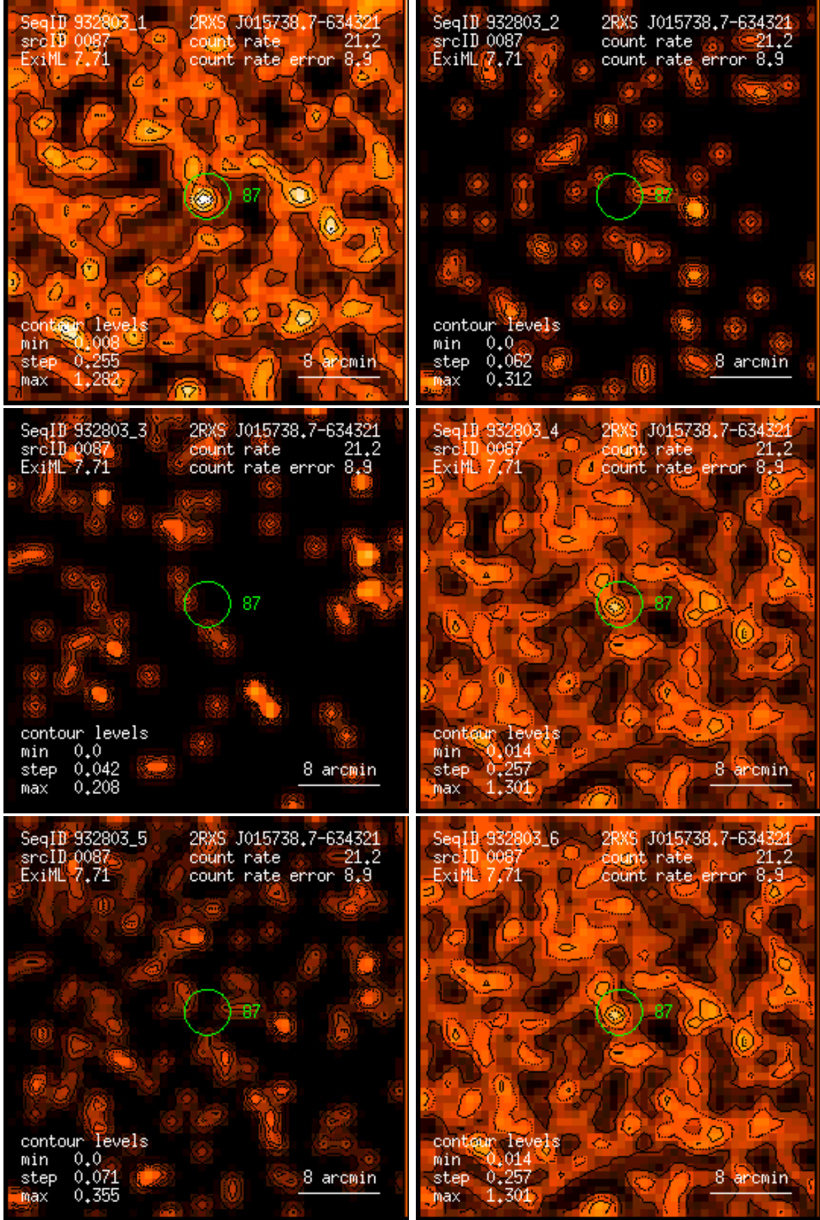
Figure 87: RASS 932803: detection 0087: band rate images, Gaussian filter: (1) PSPC channels 11 – 41, (2) 52 – 90, (3) 91 – 201, (4) 11 – 235, (5) 52 – 201, (6) 11 – 201. Broad band rates in counts/ks. Band rate contour levels in counts/ks/arcmin 2 .
