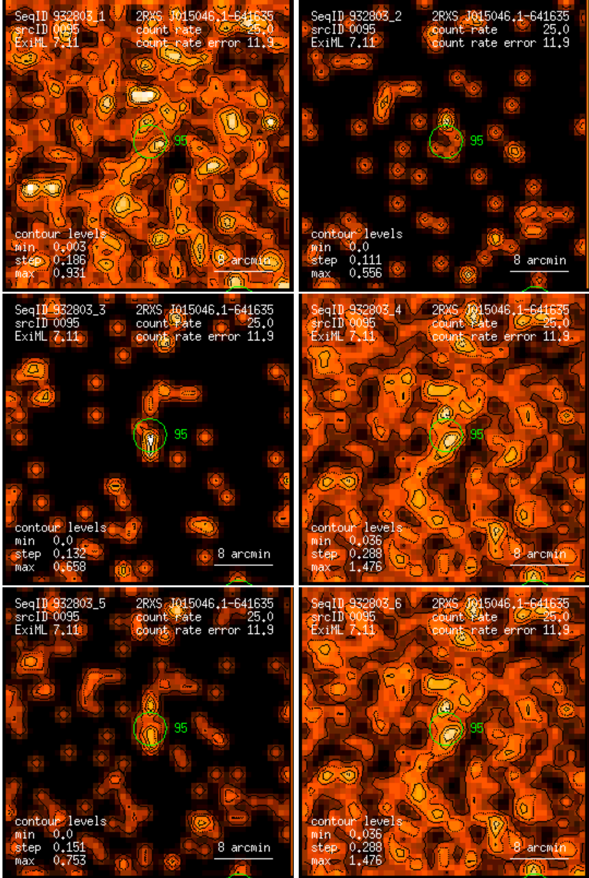
Figure 95: RASS 932803: detection 0095: band rate images, Gaussian filter: (1) PSPC channels 11 – 41, (2) 52 – 90, (3) 91 – 201, (4) 11 – 235, (5) 52 – 201, (6) 11 – 201. Broad band rates in counts/ks. Band rate contour levels in counts/ks/arcmin 2 .
