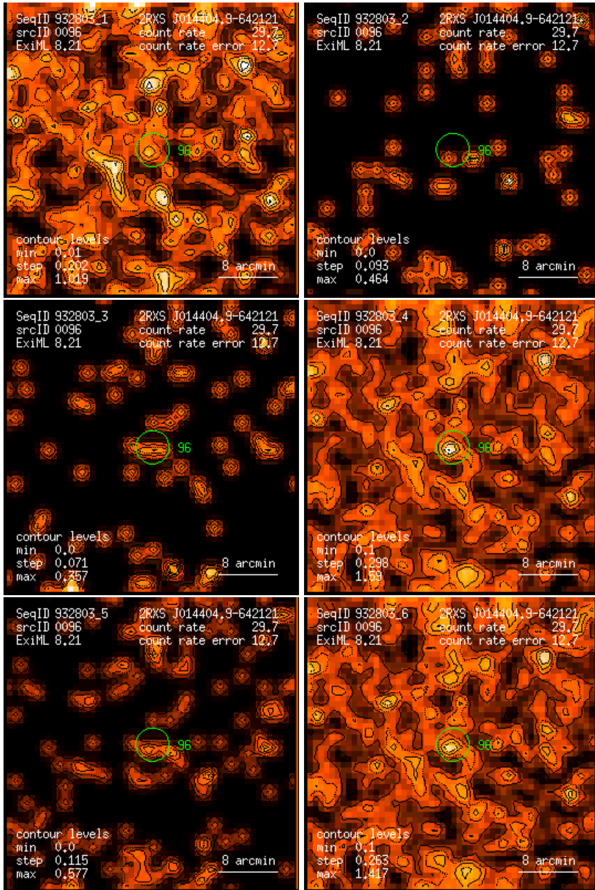
Figure 96: RASS 932803: detection 0096: band rate images, Gaussian filter: (1) PSPC channels 11 – 41, (2) 52 – 90, (3) 91 – 201, (4) 11 – 235, (5) 52 – 201, (6) 11 – 201. Broad band rates in counts/ks. Band rate contour levels in counts/ks/arcmin 2 .
