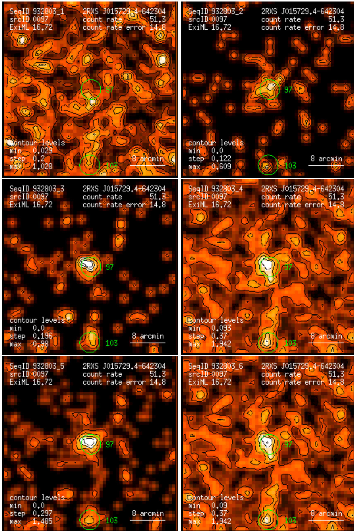
Figure 97: RASS 932803: detection 0097: band rate images, Gaussian filter: (1) PSPC channels 11 – 41, (2) 52 – 90, (3) 91 – 201, (4) 11 – 235, (5) 52 – 201, (6) 11 – 201. Broad band rates in counts/ks. Band rate contour levels in counts/ks/arcmin 2 .
