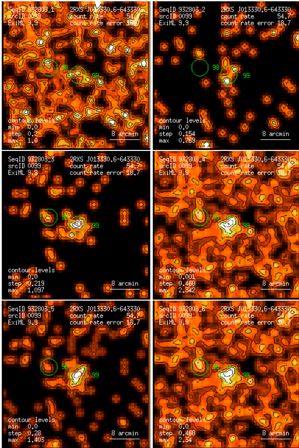
Figure 99: RASS 932803: detection 0099: band rate images, Gaussian filter: (1) PSPC channels 11 – 41, (2) 52 – 90, (3) 91 – 201, (4) 11 – 235, (5) 52 – 201, (6) 11 – 201. Broad band rates in counts/ks. Band rate contour levels in counts/ks/arcmin 2 .
