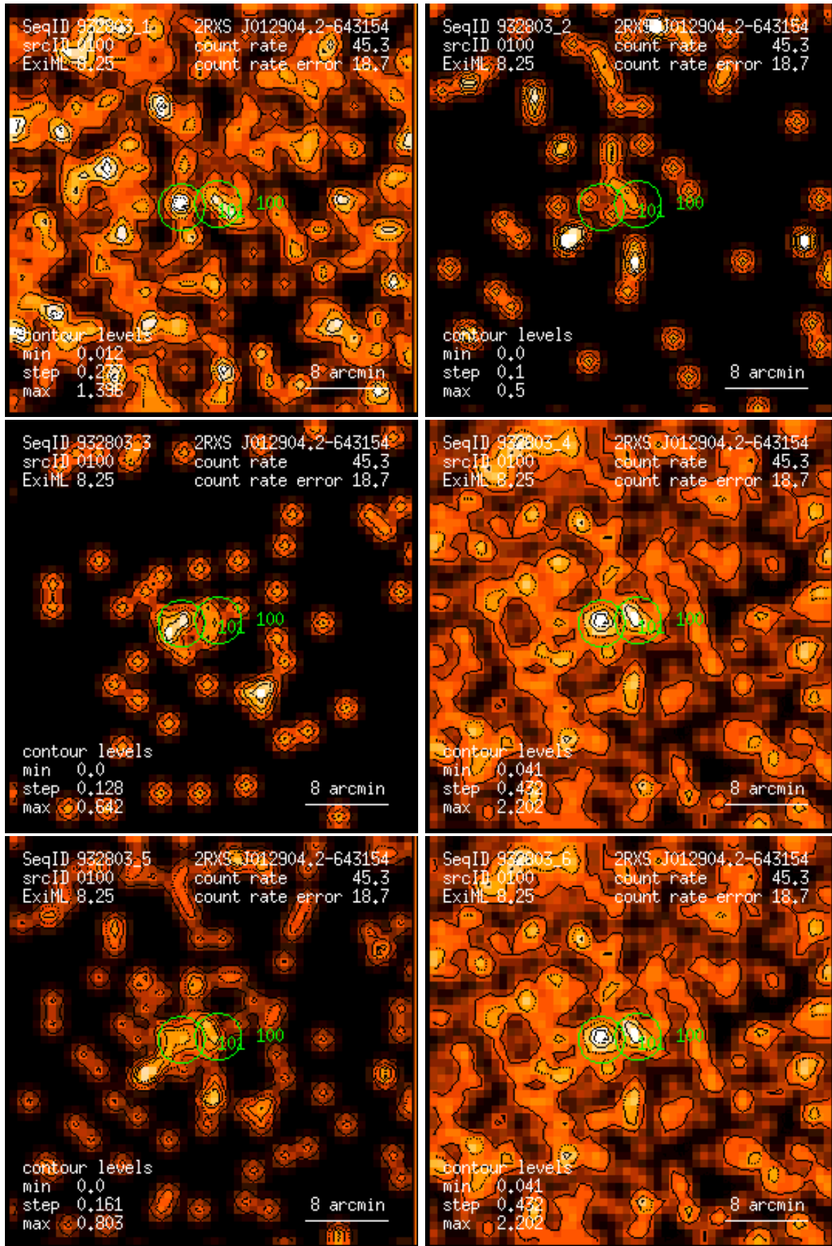
Figure 100: RASS 932803: detection 0100: band rate images, Gaussian filter: (1) PSPC channels 11 – 41, (2) 52 – 90, (3) 91 – 201, (4) 11 – 235, (5) 52 – 201, (6) 11 – 201. Broad band rates in counts/ks. Band rate contour levels in counts/ks/arcmin 2 .
