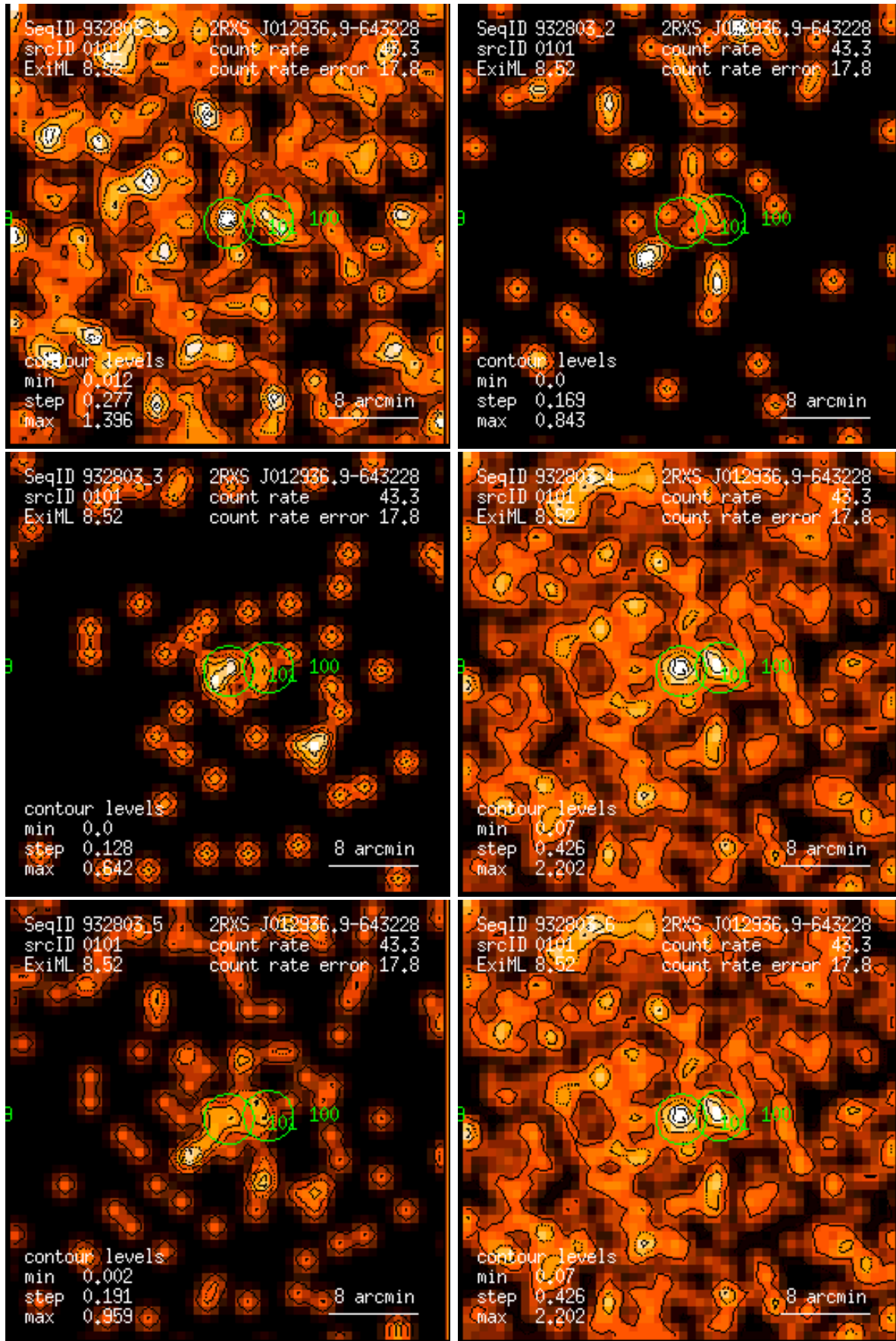
Figure 101: RASS 932803: detection 0101: band rate images, Gaussian filter: (1) PSPPC channels 11 – 41, (2) 52 – 90, (3) 91 – 201, (4) 11 – 235, (5) 52 – 201, (6) 11 – 201. Broad band rates in counts/ks. Band rate contour levels in counts/ks/arcmin 2 .
