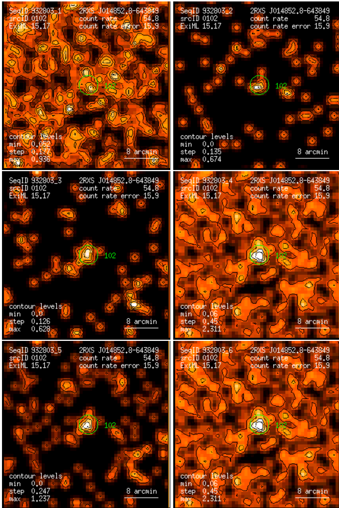
Figure 102: RASS 932803: detection 0102: band rate images, Gaussian filter: (1) PSPC channels 11 – 41, (2) 52 – 90, (3) 91 – 201, (4) 11 – 235, (5) 52 – 201, (6) 11 – 201. Broad band rates in counts/ks. Band rate contour levels in counts/ks/arcmin 2 .
