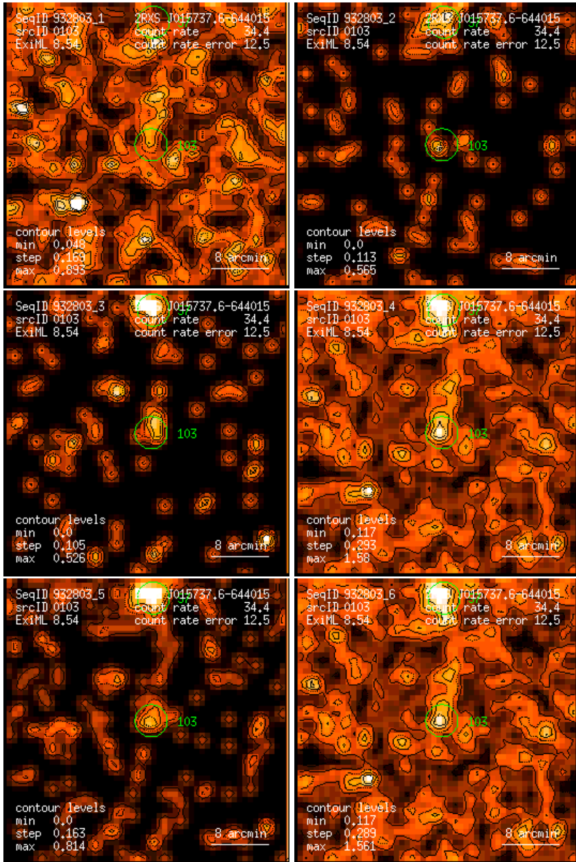
Figure 103: RASS 932803: detection 0103: band rate images, Gaussian filter: (1) PSPC channels 11 – 41, (2) 52 – 90, (3) 91 – 201, (4) 11 – 235, (5) 52 – 201, (6) 11 – 201. Broad band rates in counts/ks. Band rate contour levels in counts/ks/arcmin 2 .
