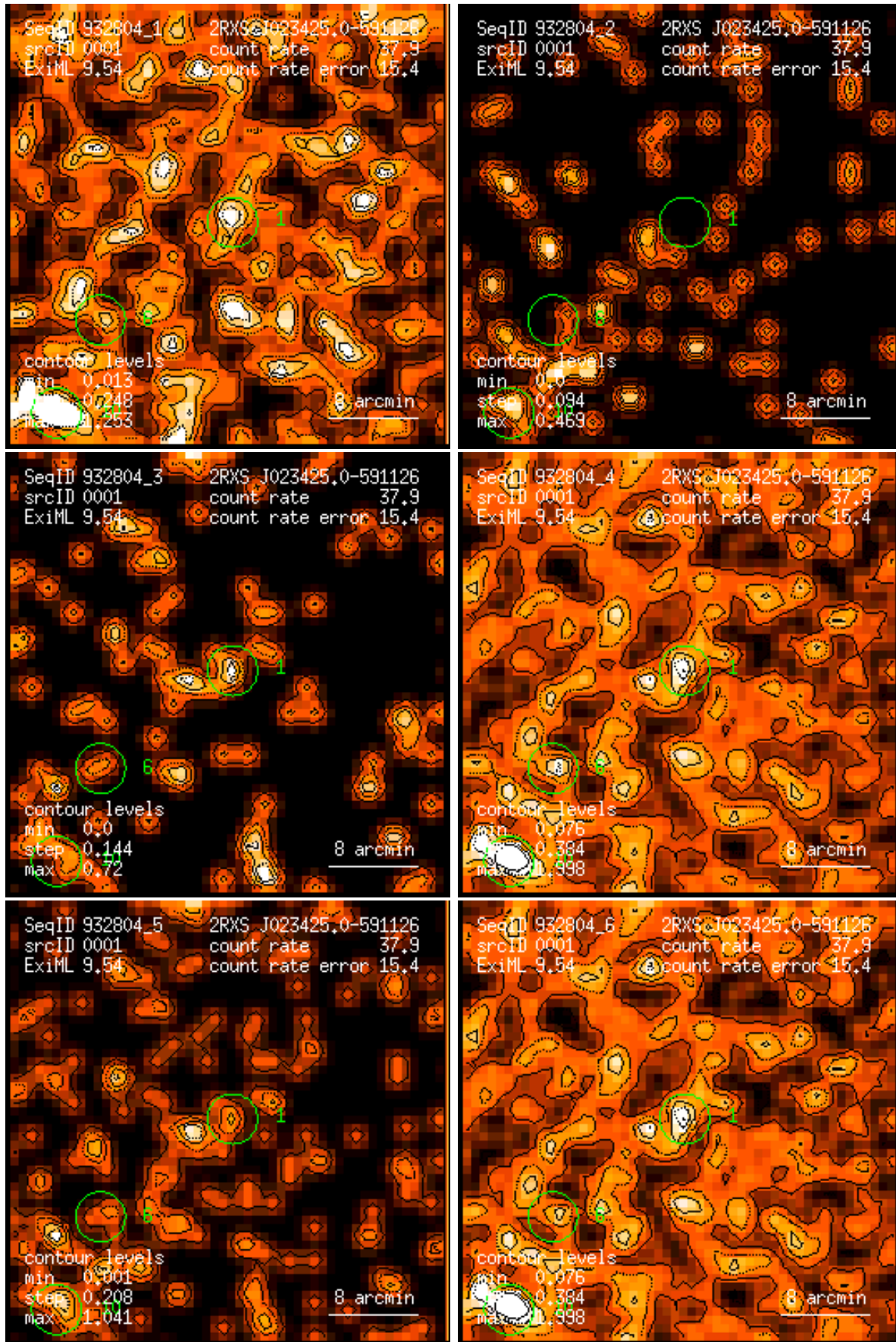
Figure 1: RASS 932804: detection 0001: band rate images, Gaussian filter: (1) PSPC channels 11 – 41, (2) 52 – 90, (3) 91 – 201, (4) 11 – 235, (5) 52 – 201, (6) 11 – 201. Broad band rates in counts/ks. Band rate contour levels in counts/ks/arcmin 2 .
