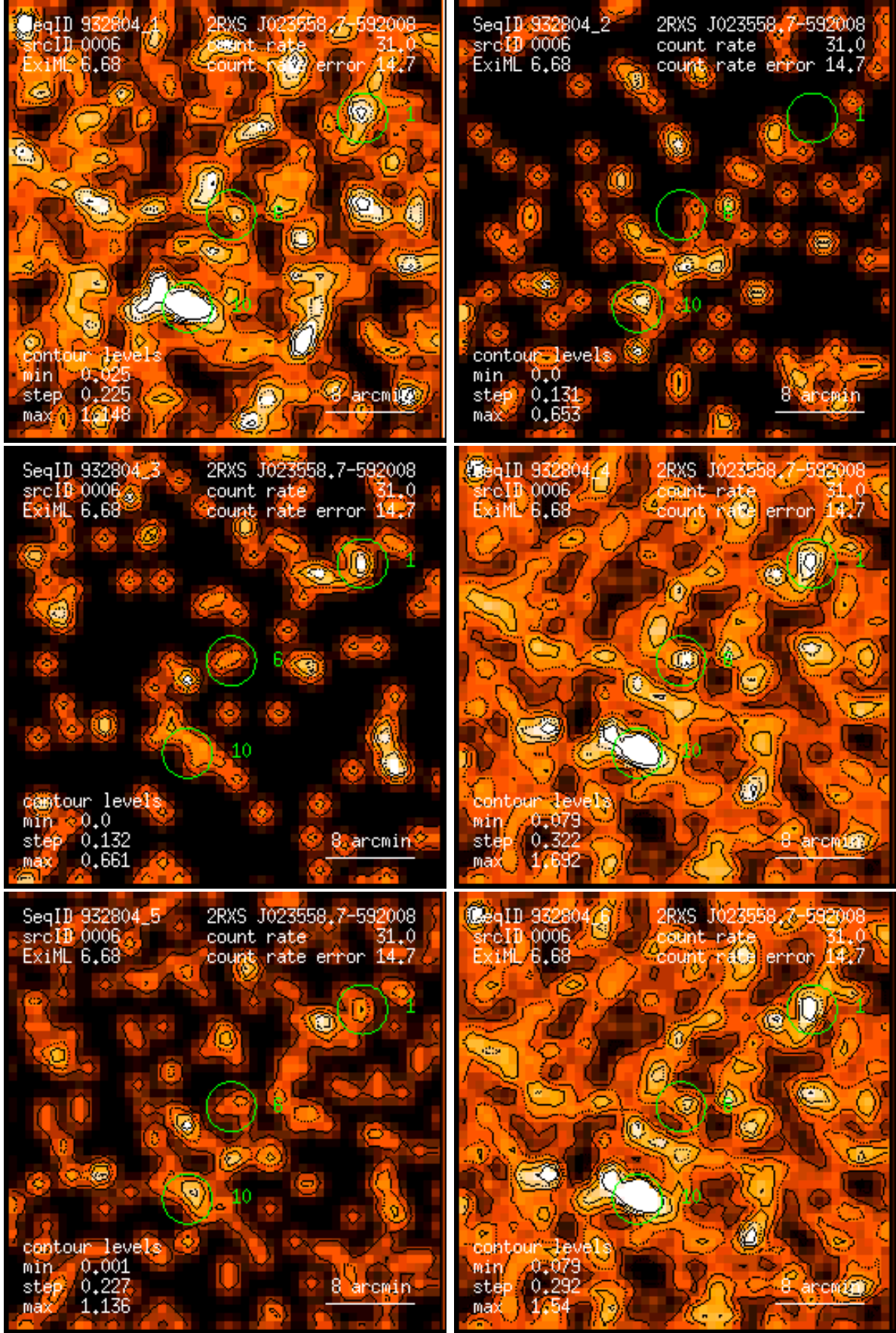
Figure 6: RASS 932804: detection 0006: band rate images, Gaussian filter: (1) PSPC channels 11 – 41, (2) 52 – 90, (3) 91 – 201, (4) 11 – 235, (5) 52 – 201, (6) 11 – 201. Broad band rates in counts/ks. Band rate contour levels in counts/ks/arcmin 2 .
