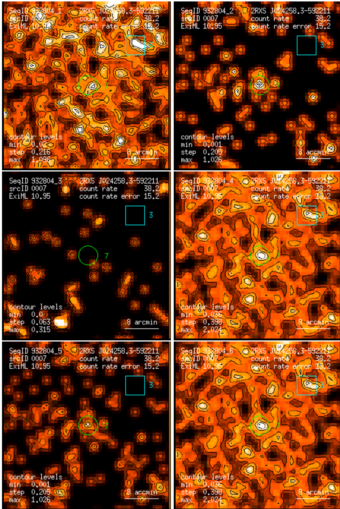
Figure 7: RASS 932804: detection 0007: band rate images, Gaussian filter: (1) PSPC channels 11 – 41, (2) 52 – 90, (3) 91 – 201, (4) 11 – 235, (5) 52 – 201, (6) 11 – 201. Broad band rates in counts/ks. Band rate contour levels in counts/ks/arcmin 2 .
