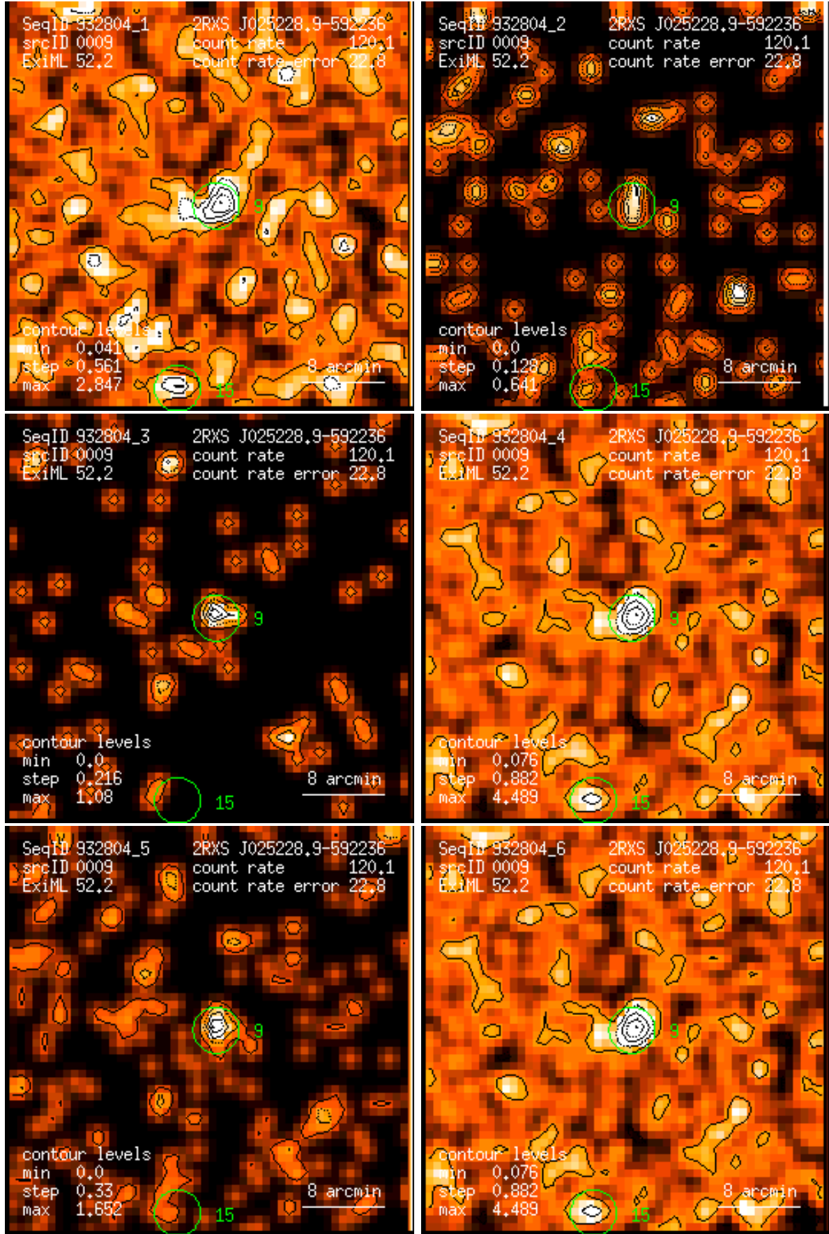
Figure 9: RASS 932804: detection 0009: band rate images, Gaussian filter: (1) PSPC channels 11 – 41, (2) 52 – 90, (3) 91 – 201, (4) 11 – 235, (5) 52 – 201, (6) 11 – 201. Broad band rates in counts/ks. Band rate contour levels in counts/ks/arcmin 2 .
