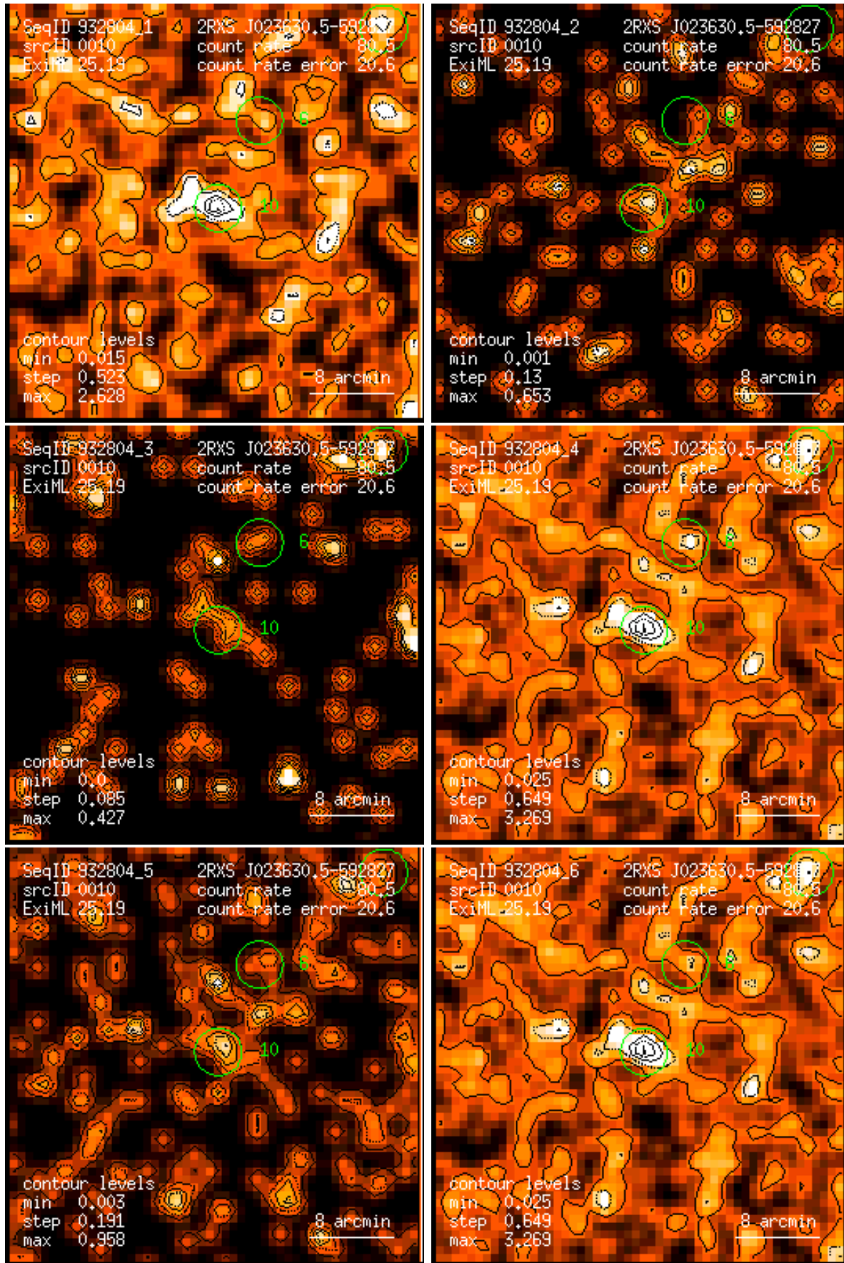
Figure 10: RASS 932804: detection 0010: band rate images, Gaussian filter: (1) PSPC channels 11 – 41, (2) 52 – 90, (3) 91 – 201, (4) 11 – 235, (5) 52 – 201, (6) 11 – 201. Broad band rates in counts/ks. Band rate contour levels in counts/ks/arcmin 2 .
