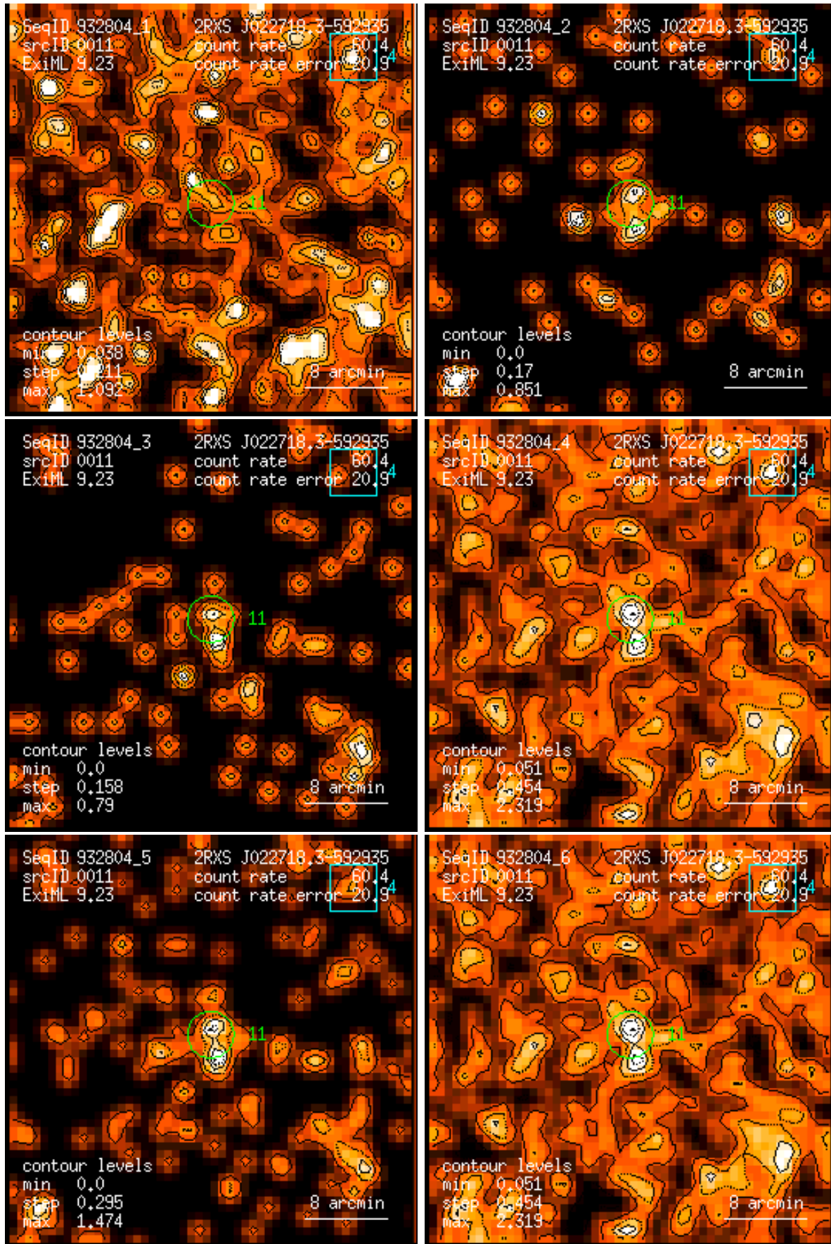
Figure 11: RASS 932804: detection 0011: band rate images, Gaussian filter: (1) PSPC channels 11 – 41, (2) 52 – 90, (3) 91 – 201, (4) 11 – 235, (5) 52 – 201, (6) 11 – 201. Broad band rates in counts/ks. Band rate contour levels in counts/ks/arcmin 2 .
