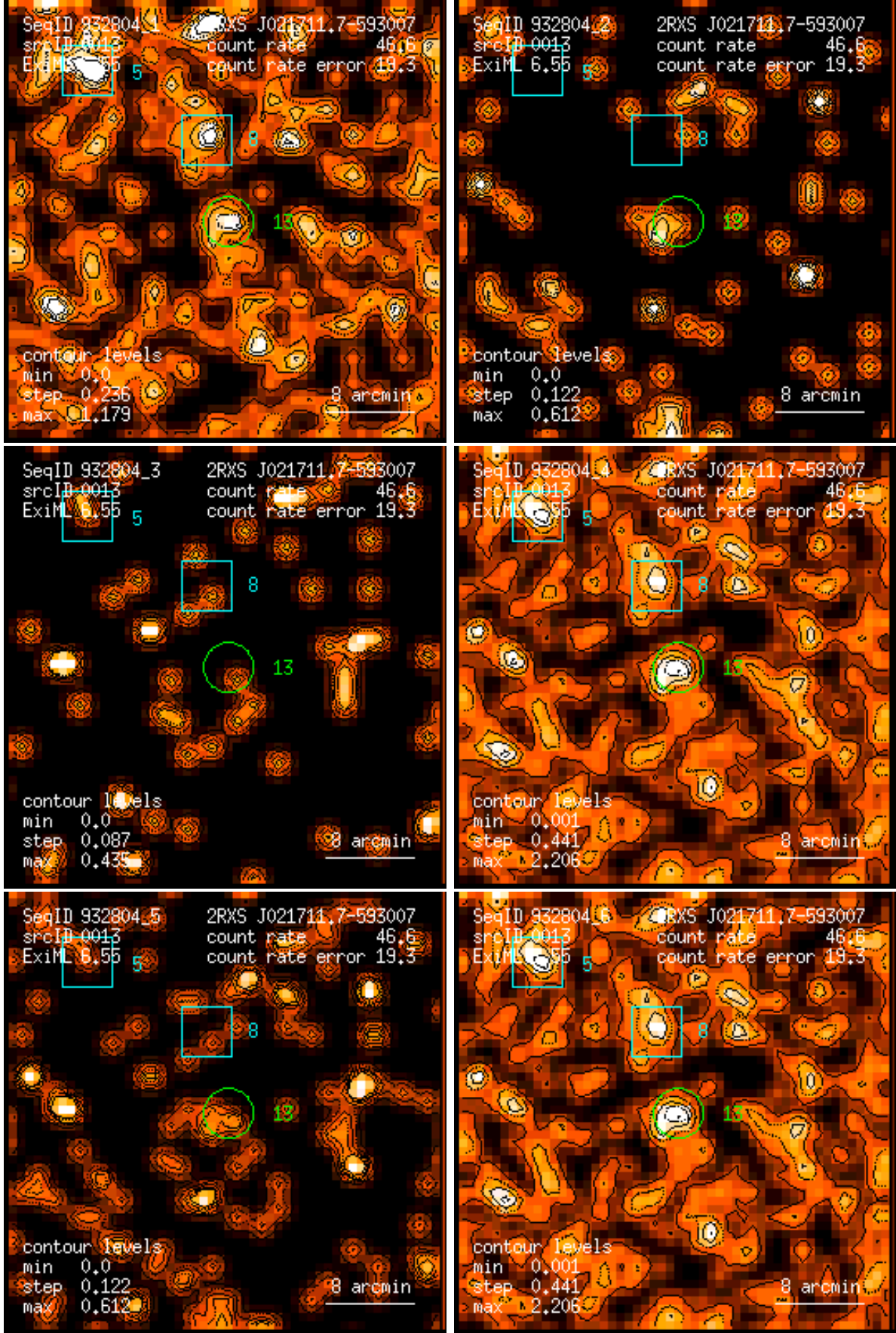
Figure 13: RASS 932804: detection 0013: band rate images, Gaussian filter: (1) PSPC channels 11 – 41, (2) 52 – 90, (3) 91 – 201, (4) 11 – 235, (5) 52 – 201, (6) 11 – 201. Broad band rates in counts/ks. Band rate contour levels in counts/ks/arcmin 2 .
