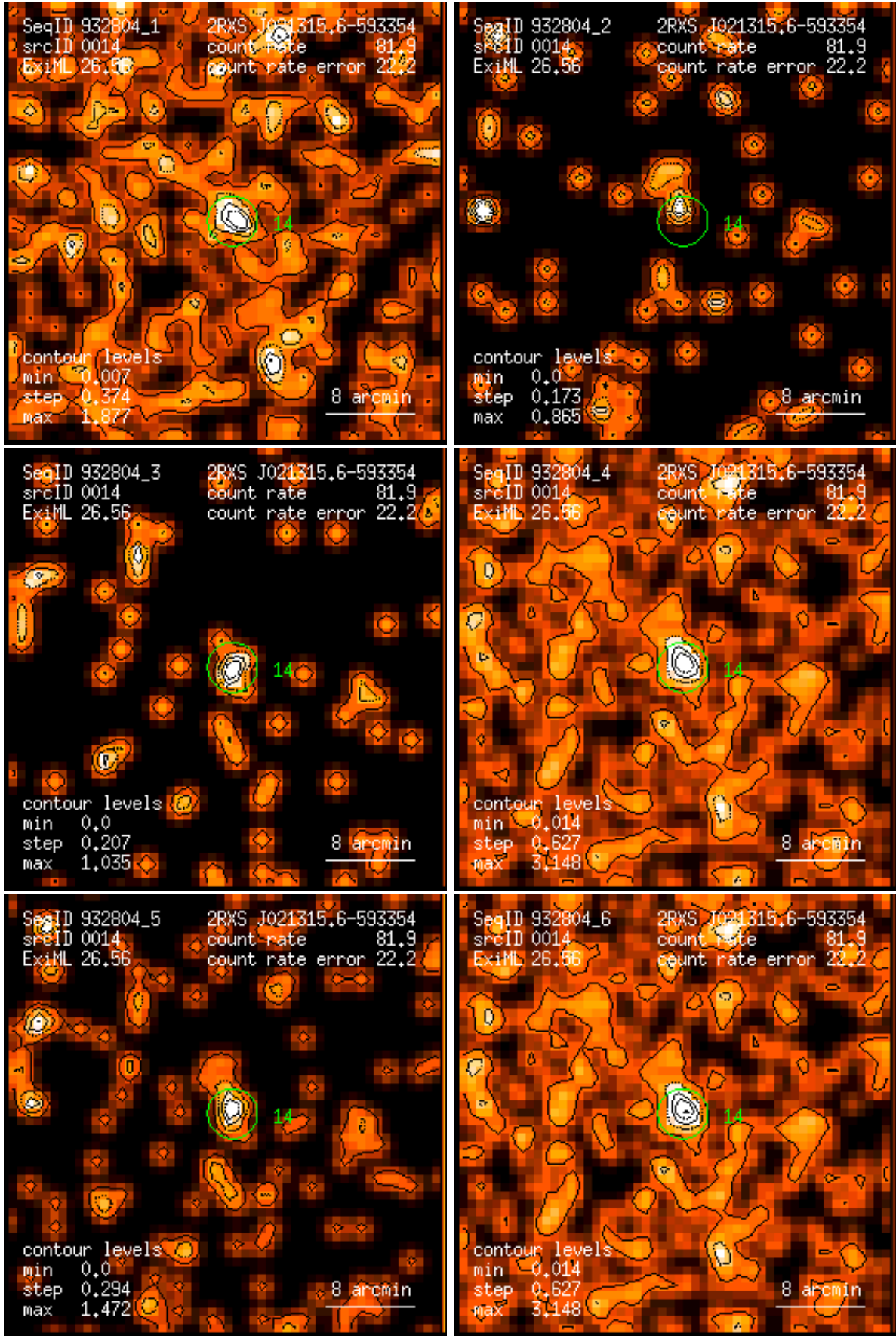
Figure 14: RASS 932804: detection 0014: band rate images, Gaussian filter: (1) PSPC channels 11 – 41, (2) 52 – 90, (3) 91 – 201, (4) 11 – 235, (5) 52 – 201, (6) 11 – 201. Broad band rates in counts/ks. Band rate contour levels in counts/ks/arcmin 2 .
