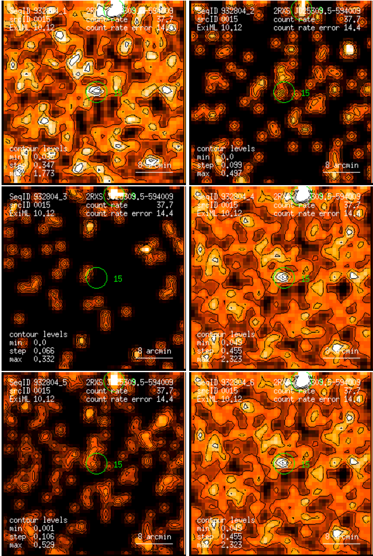
Figure 15: RASS 932804: detection 0015: band rate images, Gaussian filter: (1) PSPC channels 11 – 41, (2) 52 – 90, (3) 91 – 201, (4) 11 – 235, (5) 52 – 201, (6) 11 – 201. Broad band rates in counts/ks. Band rate contour levels in counts/ks/arcmin 2 .
