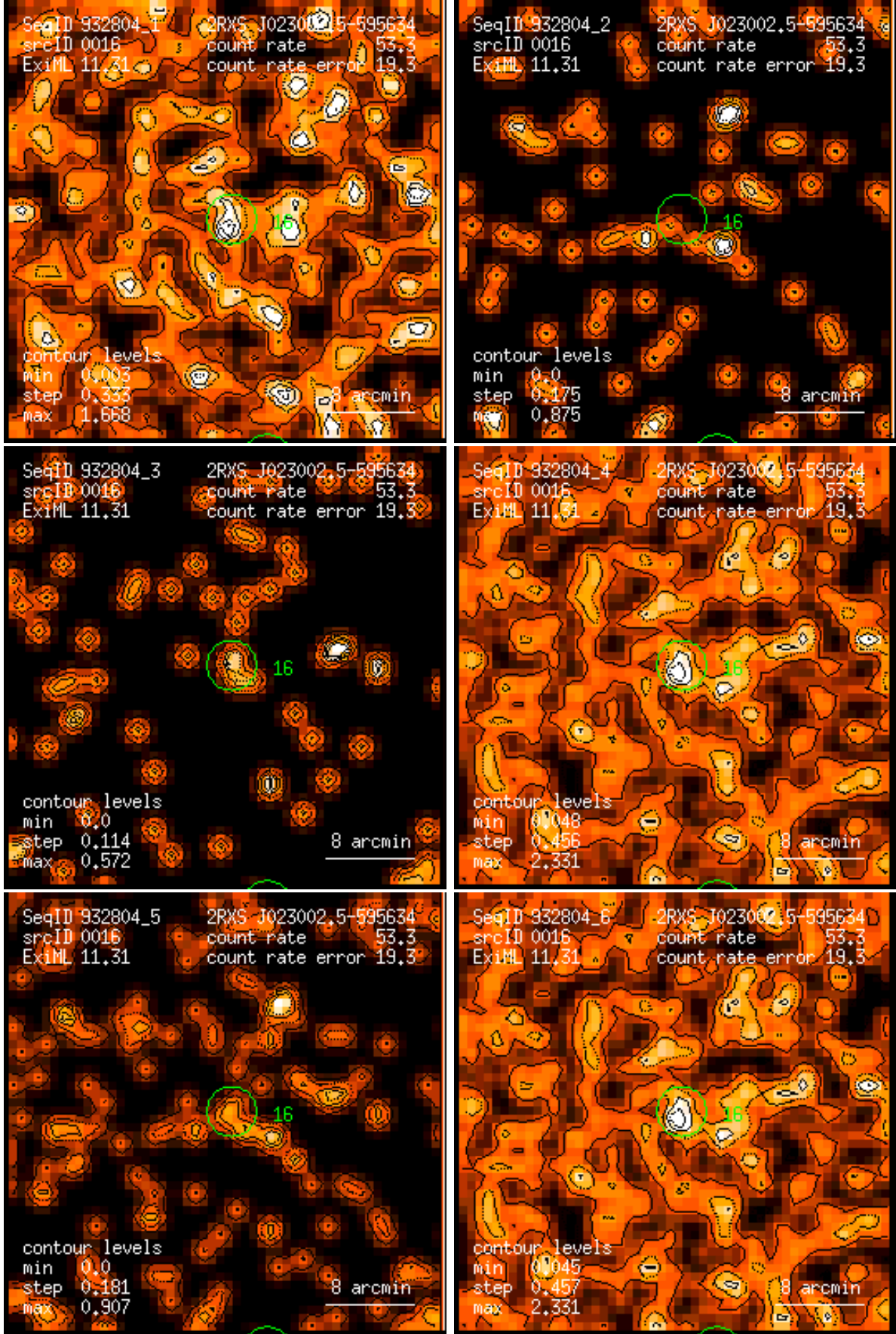
Figure 16: RASS 932804: detection 0016: band rate images, Gaussian filter: (1) PSPC channels 11 – 41, (2) 52 – 90, (3) 91 – 201, (4) 11 – 235, (5) 52 – 201, (6) 11 – 201. Broad band rates in counts/ks. Band rate contour levels in counts/ks/arcmin 2 .
