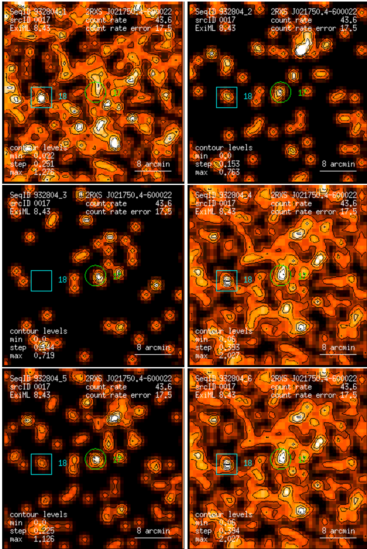
Figure 17: RASS 932804: detection 0017: band rate images, Gaussian filter: (1) PSPC channels 11 – 41, (2) 52 – 90, (3) 91 – 201, (4) 11 – 235, (5) 52 – 201, (6) 11 – 201. Broad band rates in counts/ks. Band rate contour levels in counts/ks/arcmin 2 .
