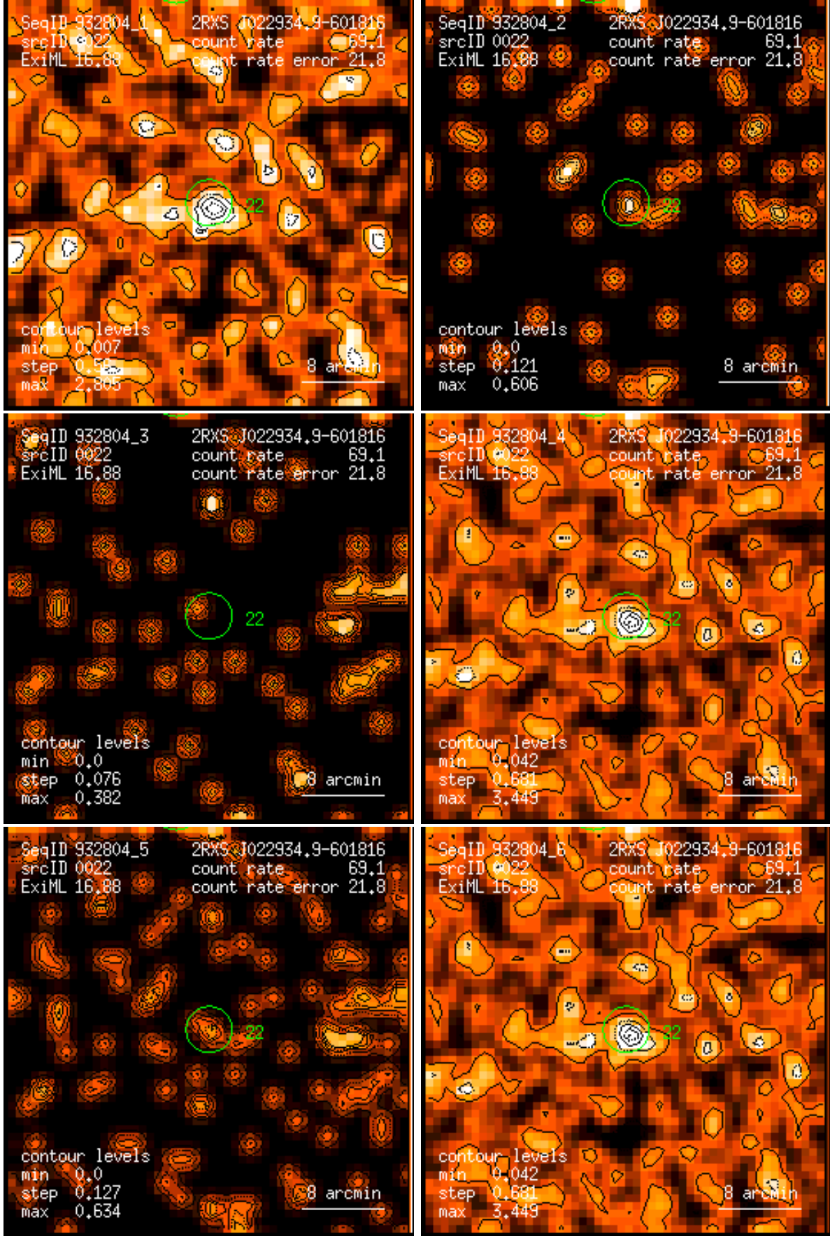
Figure 22: RASS 932804: detection 0022: band rate images, Gaussian filter: (1) PSPC channels 11 – 41, (2) 52 – 90, (3) 91 – 201, (4) 11 – 235, (5) 52 – 201, (6) 11 – 201. Broad band rates in counts/ks. Band rate contour levels in counts/ks/arcmin 2 .
