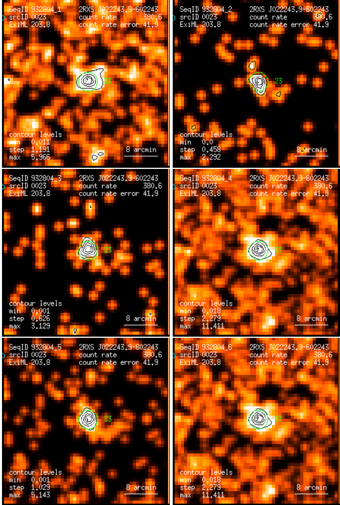
Figure 23: RASS 932804: detection 0023: band rate images, Gaussian filter: (1) PSPC channels 11 – 41, (2) 52 – 90, (3) 91 – 201, (4) 11 – 235, (5) 52 – 201, (6) 11 – 201. Broad band rates in counts/ks. Band rate contour levels in counts/ks/arcmin 2 .
