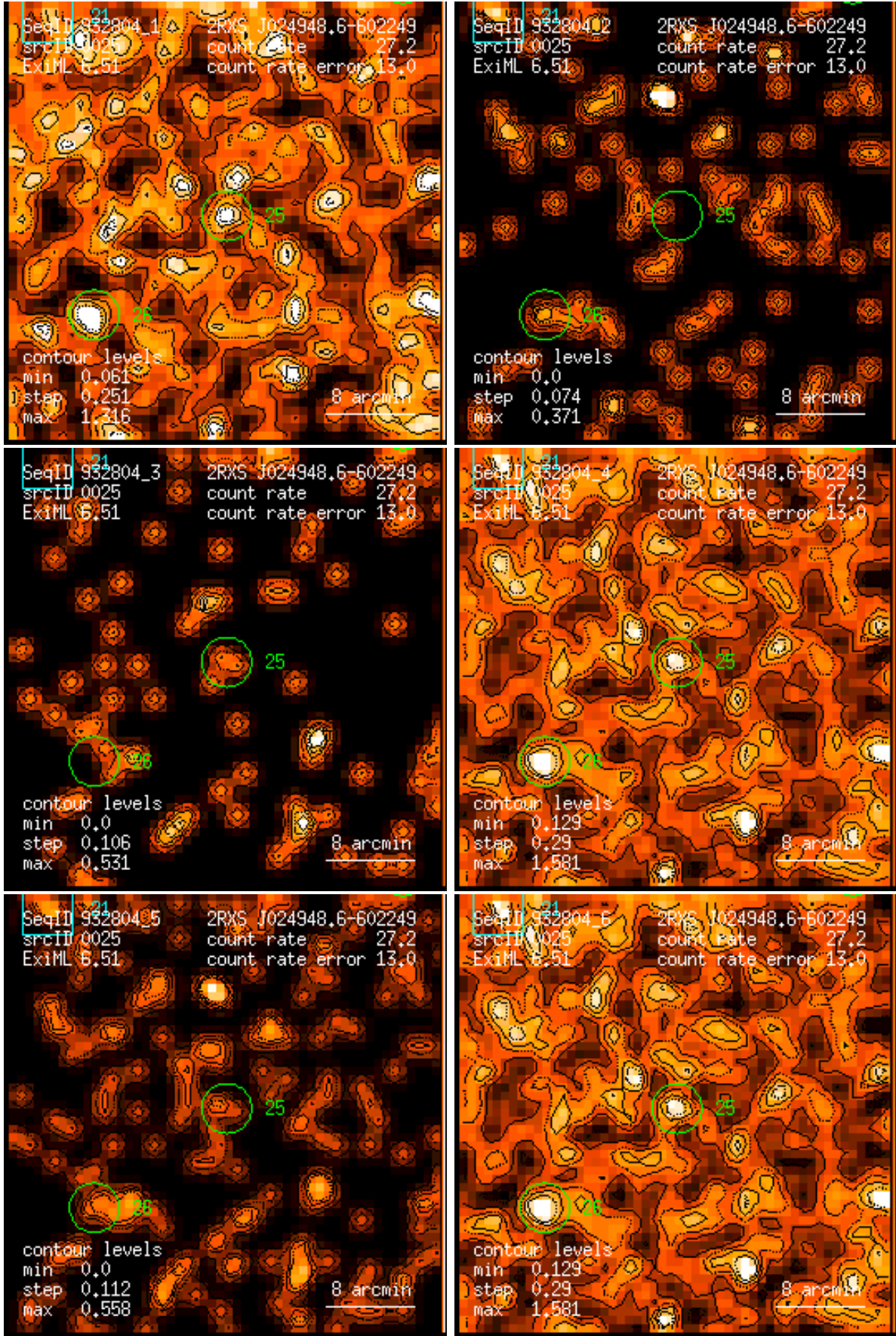
Figure 25: RASS 932804: detection 0025: band rate images, Gaussian filter: (1) PSPC channels 11 – 41, (2) 52 – 90, (3) 91 – 201, (4) 11 – 235, (5) 52 – 201, (6) 11 – 201. Broad band rates in counts/ks. Band rate contour levels in counts/ks/arcmin 2 .
