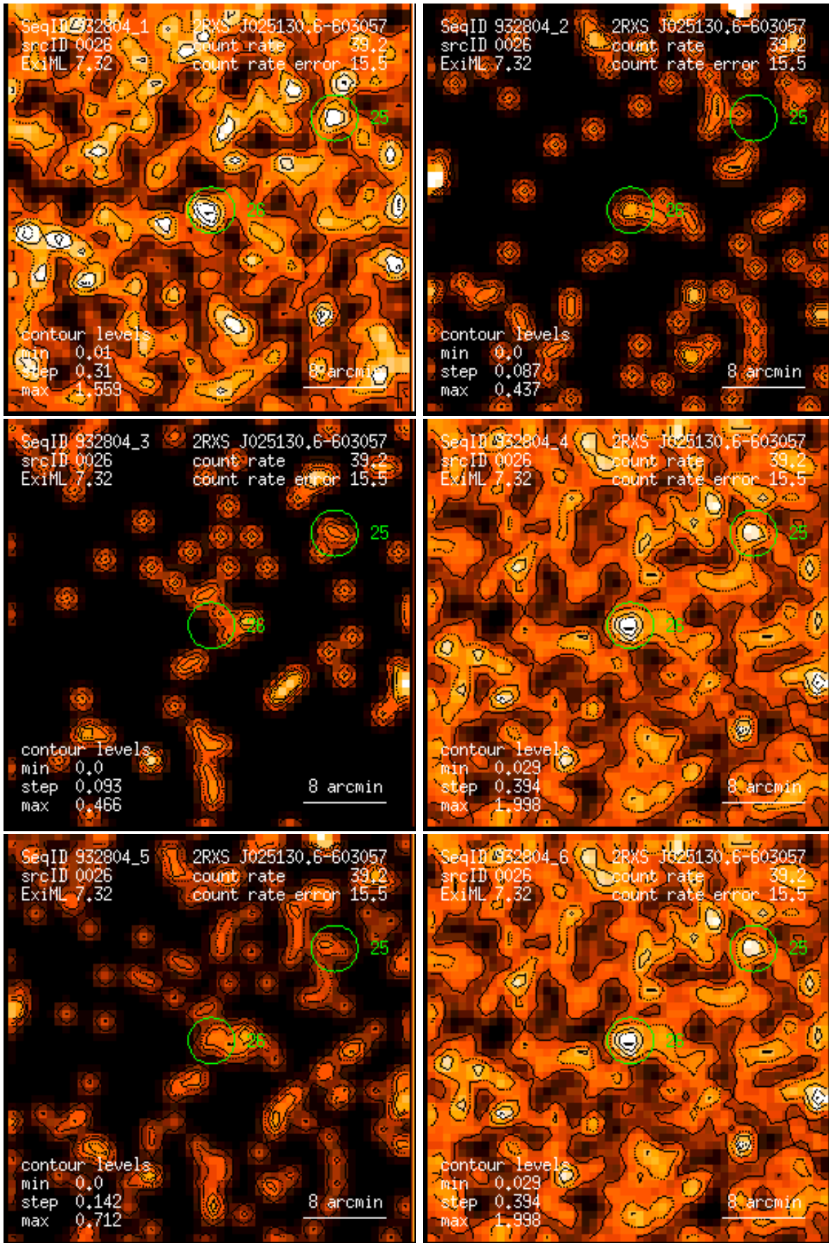
Figure 26: RASS 932804: detection 0026: band rate images, Gaussian filter: (1) PSPC channels 11 – 41, (2) 52 – 90, (3) 91 – 201, (4) 11 – 235, (5) 52 – 201, (6) 11 – 201. Broad band rates in counts/ks. Band rate contour levels in counts/ks/arcmin 2 .
