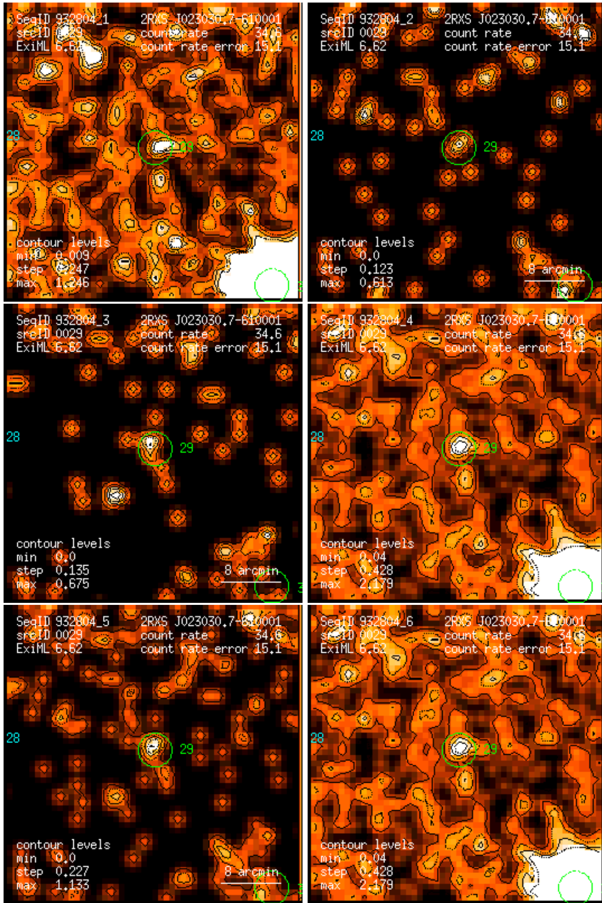
Figure 29: RASS 932804: detection 0029: band rate images, Gaussian filter: (1) PSPC channels 11 – 41, (2) 52 – 90, (3) 91 – 201, (4) 11 – 235, (5) 52 – 201, (6) 11 – 201. Broad band rates in counts/ks. Band rate contour levels in counts/ks/arcmin 2 .
