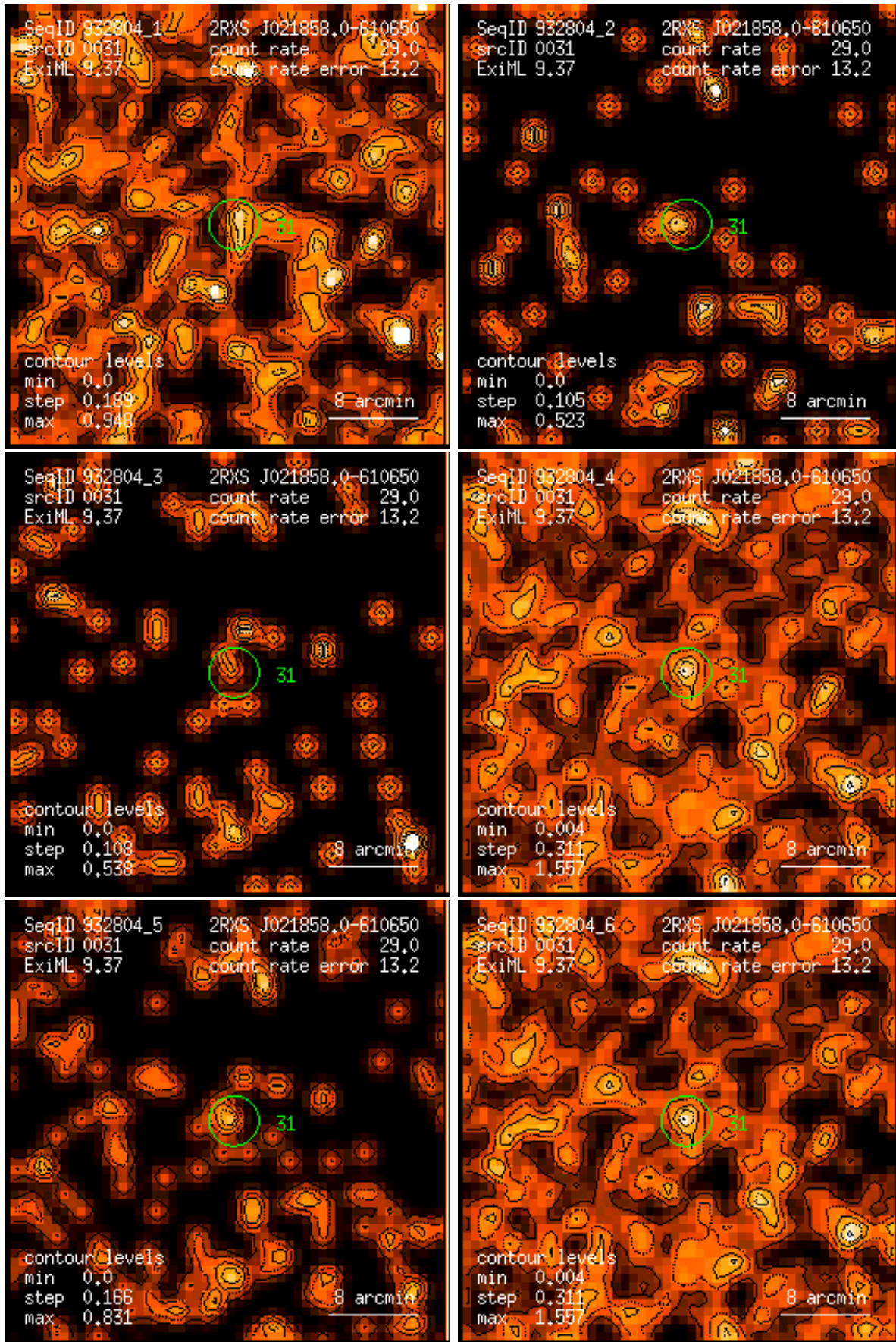
Figure 31: RASS 932804: detection 0031: band rate images, Gaussian filter: (1) PSPC channels 11 – 41, (2) 52 – 90, (3) 91 – 201, (4) 11 – 235, (5) 52 – 201, (6) 11 – 201. Broad band rates in counts/ks. Band rate contour levels in counts/ks/arcmin 2 .
