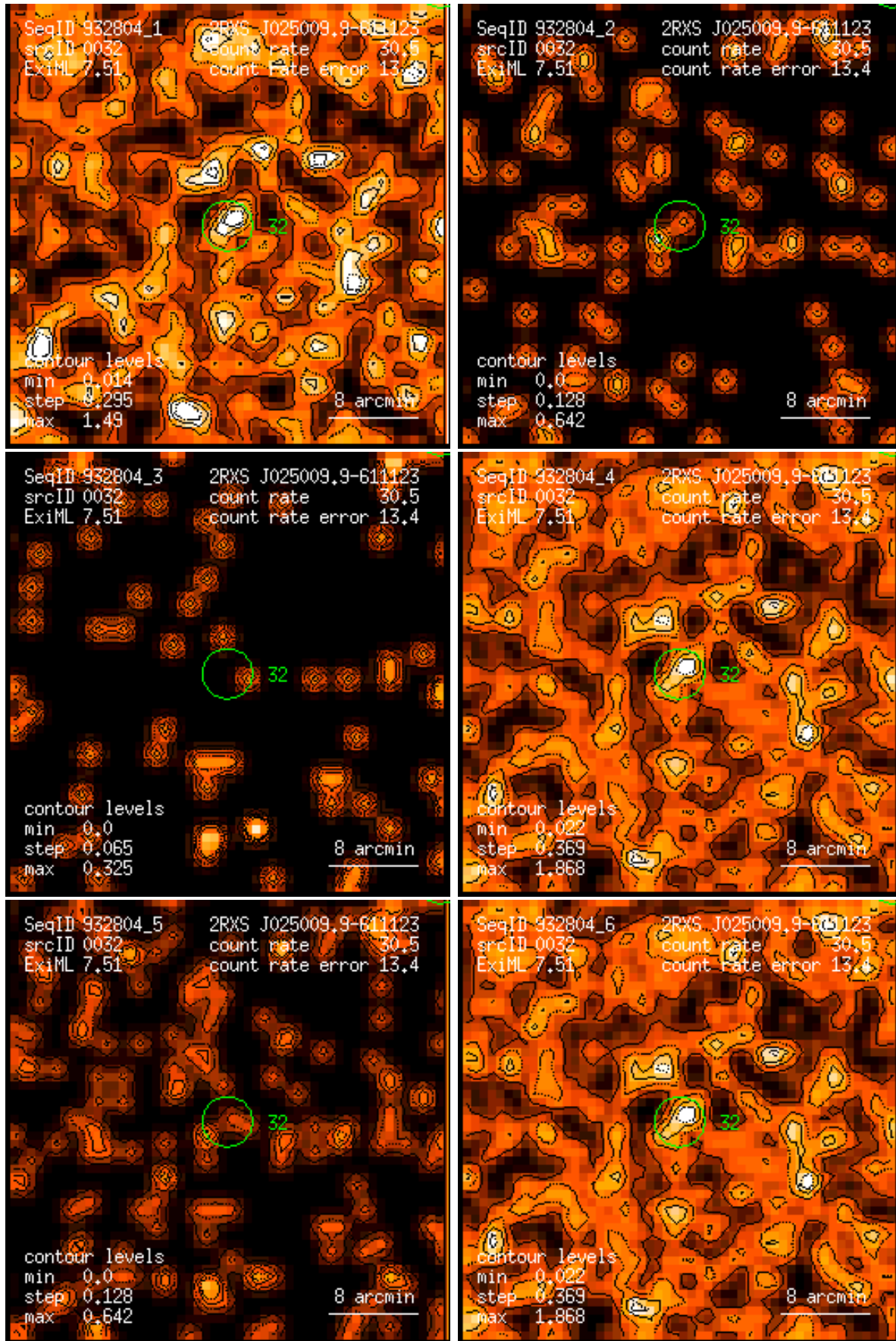
Figure 32: RASS 932804: detection 0032: band rate images, Gaussian filter: (1) PSPC channels 11 – 41, (2) 52 – 90, (3) 91 – 201, (4) 11 – 235, (5) 52 – 201, (6) 11 – 201. Broad band rates in counts/ks. Band rate contour levels in counts/ks/arcmin 2 .
