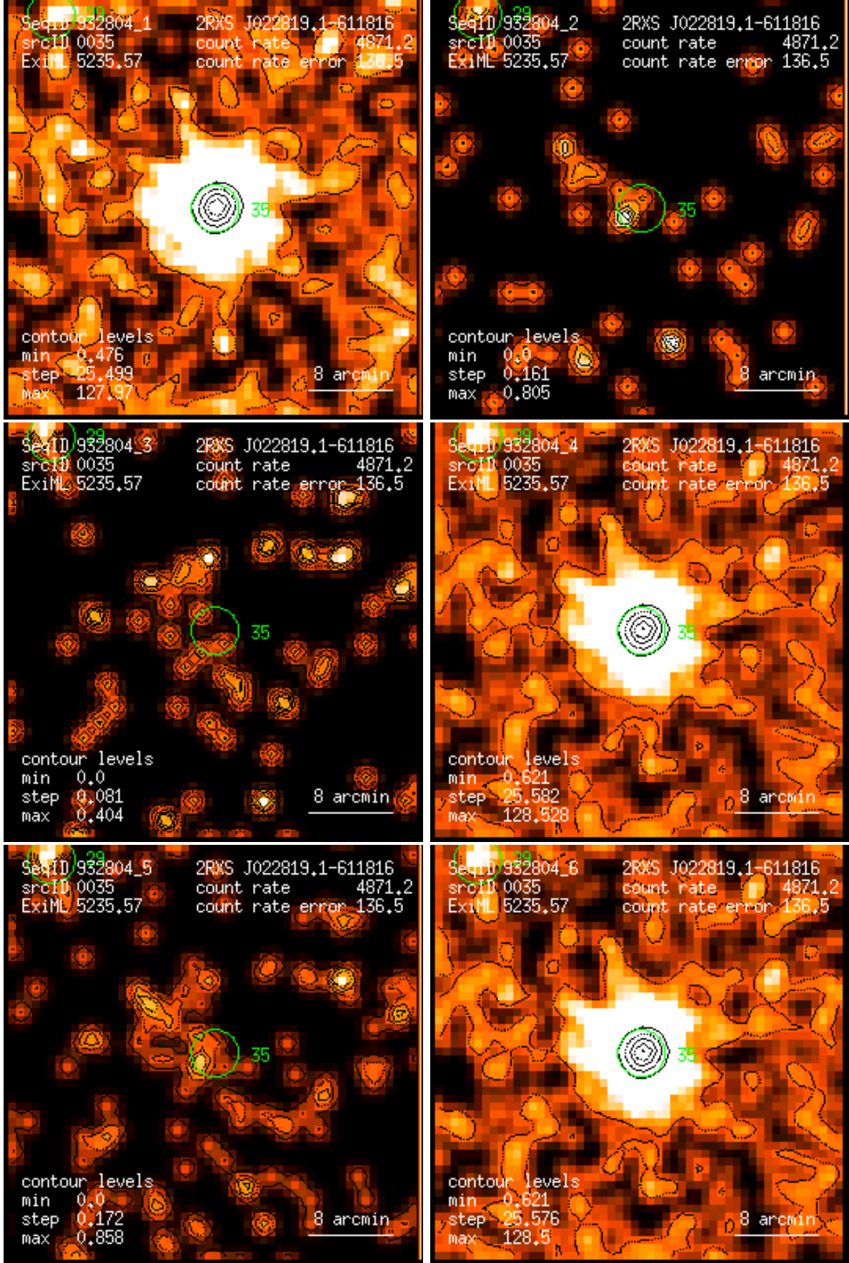
Figure 35: RASS 932804: detection 0035: band rate images, Gaussian filter: (1) PSPC channels 11 – 41, (2) 52 – 90, (3) 91 – 201, (4) 11 – 235, (5) 52 – 201, (6) 11 – 201. Broad band rates in counts/ks. Band rate contour levels in counts/ks/arcmin 2 .
