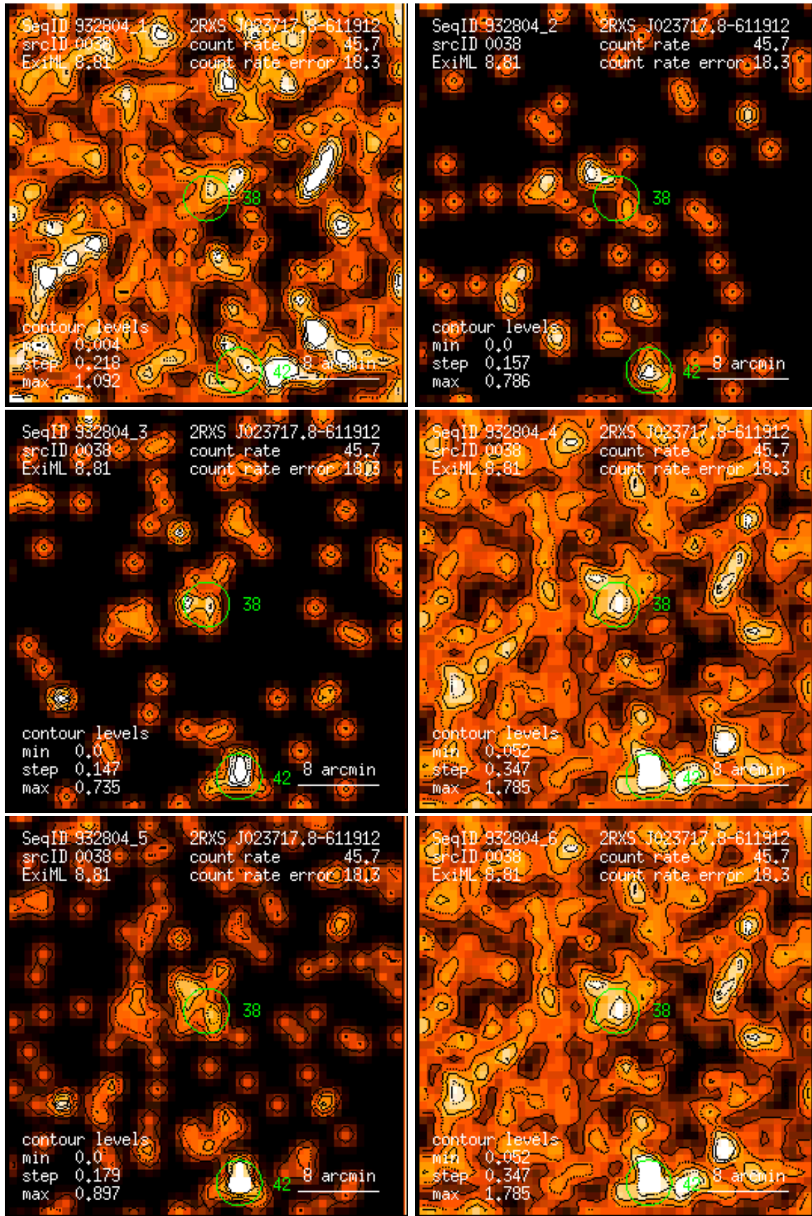
Figure 38: RASS 932804: detection 0038: band rate images, Gaussian filter: (1) PSPC channels 11 – 41, (2) 52 – 90, (3) 91 – 201, (4) 11 – 235, (5) 52 – 201, (6) 11 – 201. Broad band rates in counts/ks. Band rate contour levels in counts/ks/arcmin 2 .
