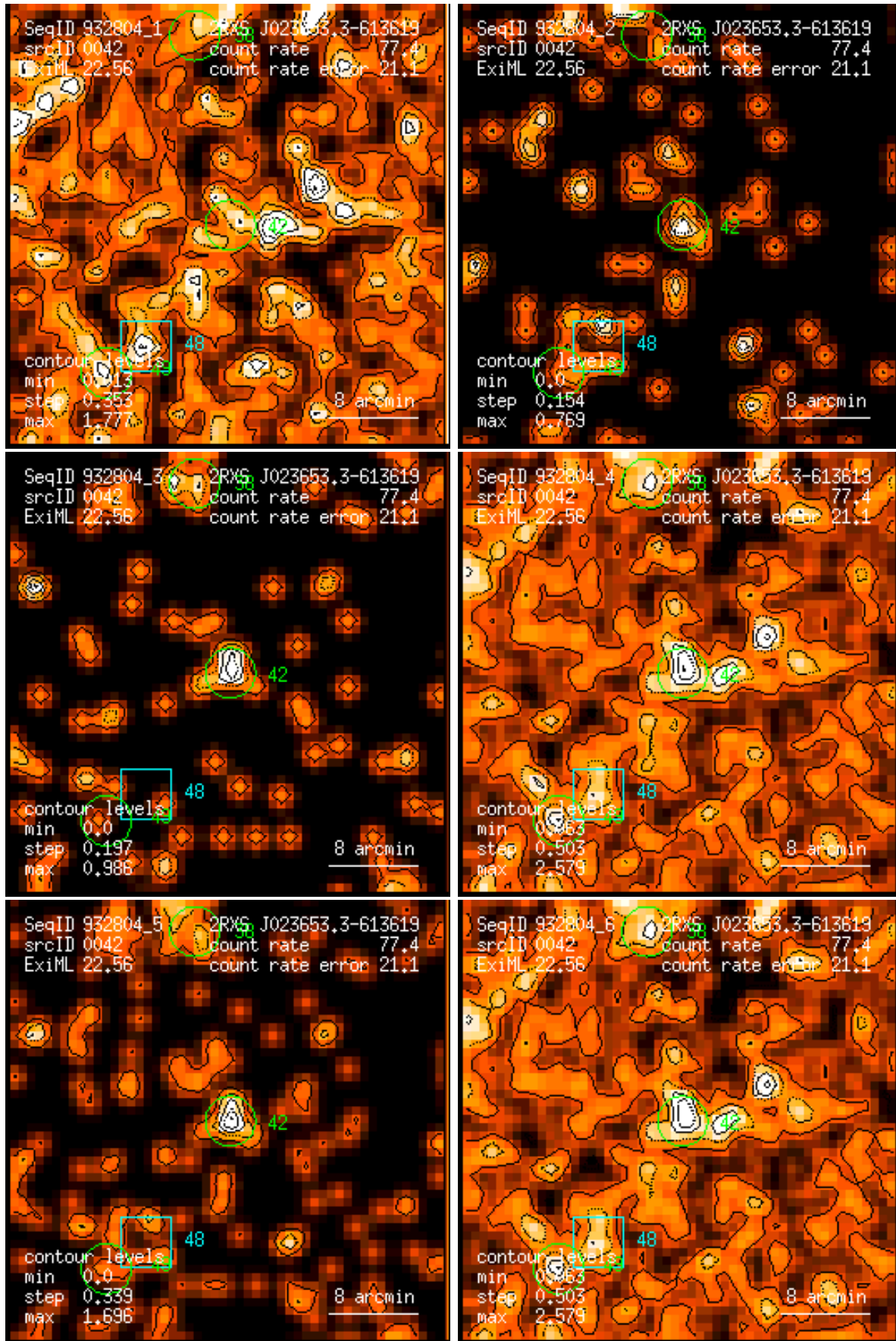
Figure 42: RASS 932804: detection 0042: band rate images, Gaussian filter: (1) PSPC channels 11 – 41, (2) 52 – 90, (3) 91 – 201, (4) 11 – 235, (5) 52 – 201, (6) 11 – 201. Broad band rates in counts/ks. Band rate contour levels in counts/ks/arcmin 2 .
