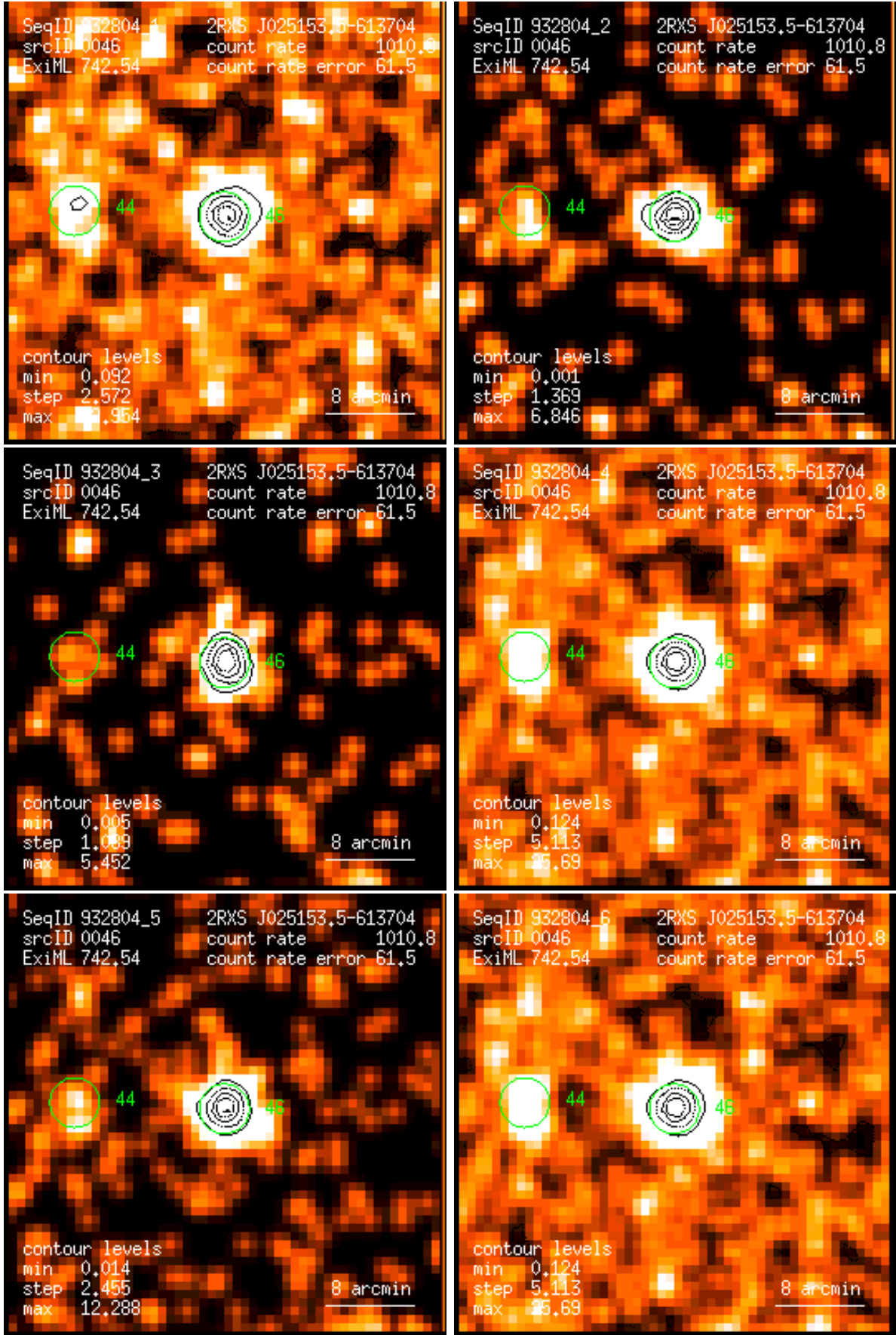
Figure 46: RASS 932804: detection 0046: band rate images, Gaussian filter: (1) PSPC channels 11 – 41, (2) 52 – 90, (3) 91 – 201, (4) 11 – 235, (5) 52 – 201, (6) 11 – 201. Broad band rates in counts/ks. Band rate contour levels in counts/ks/arcmin 2 .
