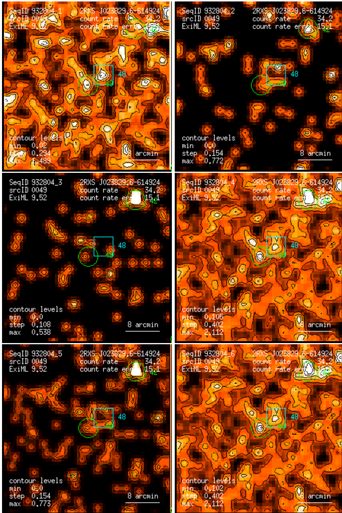
Figure 49: RASS 932804: detection 0049: band rate images, Gaussian filter: (1) PSPC channels 11 – 41, (2) 52 – 90, (3) 91 – 201, (4) 11 – 235, (5) 52 – 201, (6) 11 – 201. Broad band rates in counts/ks. Band rate contour levels in counts/ks/arcmin 2 .
