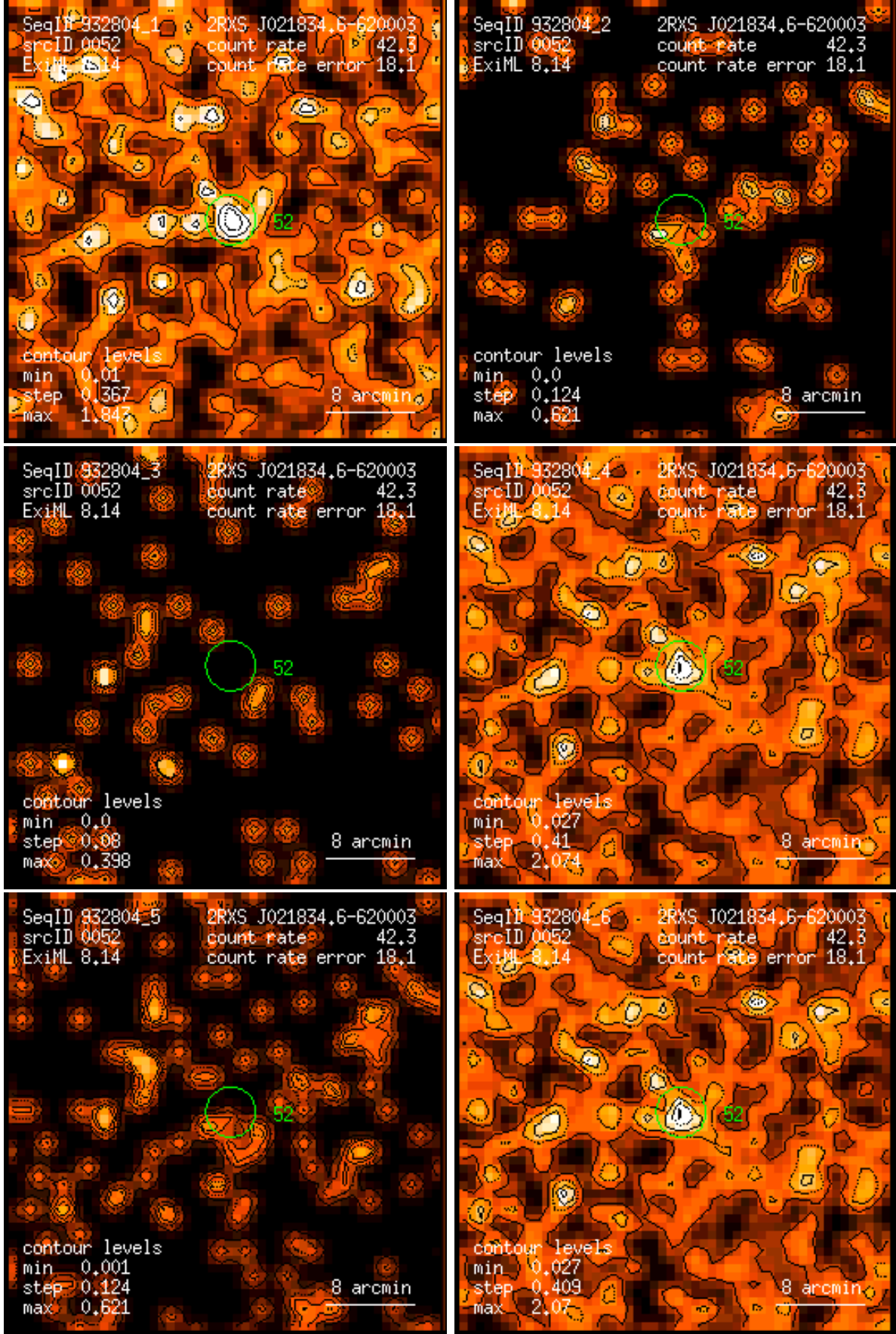
Figure 52: RASS 932804: detection 0052: band rate images, Gaussian filter: (1) PSPC channels 11 – 41, (2) 52 – 90, (3) 91 – 201, (4) 11 – 235, (5) 52 – 201, (6) 11 – 201. Broad band rates in counts/ks. Band rate contour levels in counts/ks/arcmin 2 .
